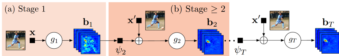
Figure 2-46 : The improved Convolutional Pose Machines of Wei et al. [2016] integrate the prediction and refinement stages within a unified architecture that can be trained end-to-end, resulting in large performance improvements.
