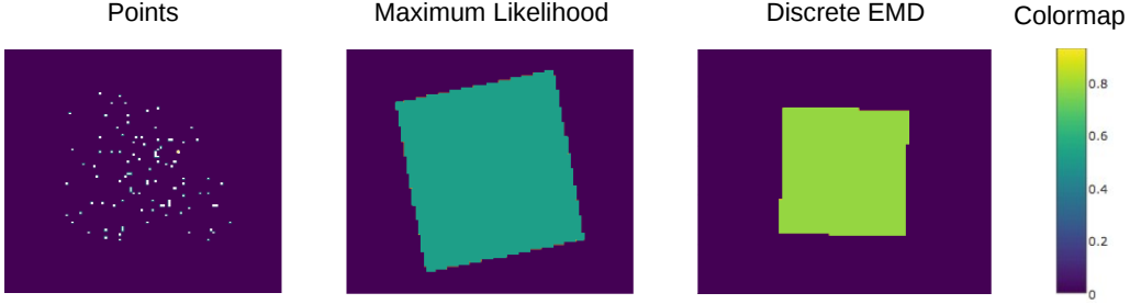
Figure D-7: We fit the uniform rectangle to our data by optimizing the Maximum Likelihood of the points under the rectangle model, and the EMD distance. EMD is computed using Euclidean distance on the 2D plane.
