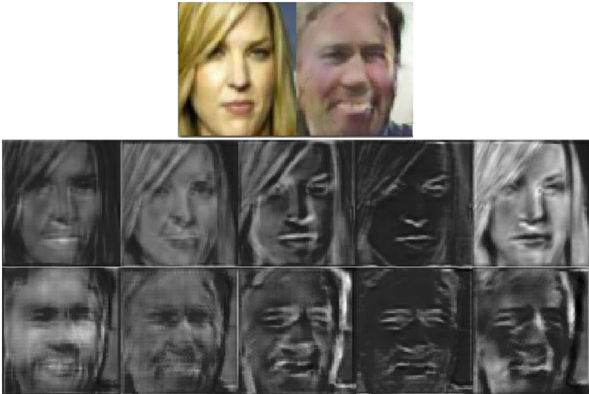
Figure 5-6: First row: Face from the training dataset (left) and face generated by a Deep Convolutional GAN (right). Second row: output maps of the first convolution layer for the real face. Third row: same output maps for the generated face. While the generated face does not show visible artifacts, some appear clearly as horizontal and vertical lines, especially on the two leftmost maps.
