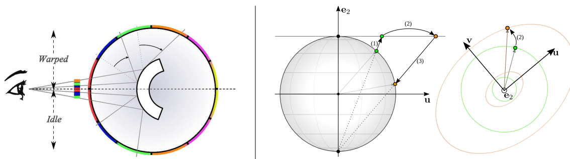
Figure 3.4: Left: the depicted curvature is exaggerated through reflected light patterns by expanding the region that is reflected off the surface (curving arrows), which in turn compresses reflections on the object compared to rendering without warping ('idle'). Right: The warping process modifies the light direction by (1) stereographic projection, followed by (2) scaling to a new position in stereographic space and (3) inverse stereographic projection back to the sphere of directions. The effect of principal curvature directions in step (2) is visualized in the stereographic plane: scaling maps projected lighting directions from the green circles to the orange ellipses.
