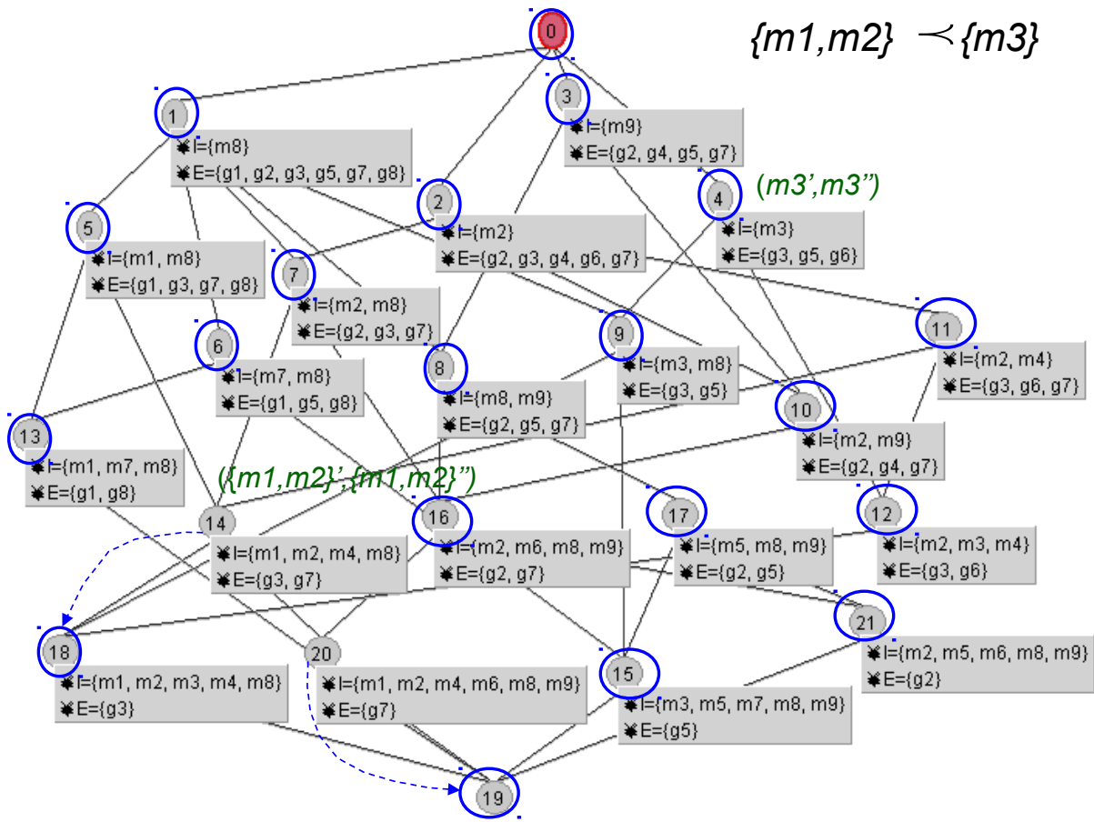
Figure 4.10: The lattice constrained by \{m1, m2\} < \{m3\} and the trace of changes.
