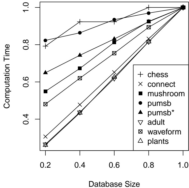
Figure 10.1: Scalability of Σοφία w.r.t. dataset size. X-axis shows the fraction of objects taken from an original dataset, and Y-axis shows the fraction of time w.r.t. the computational time needed for processing the original dataset.
