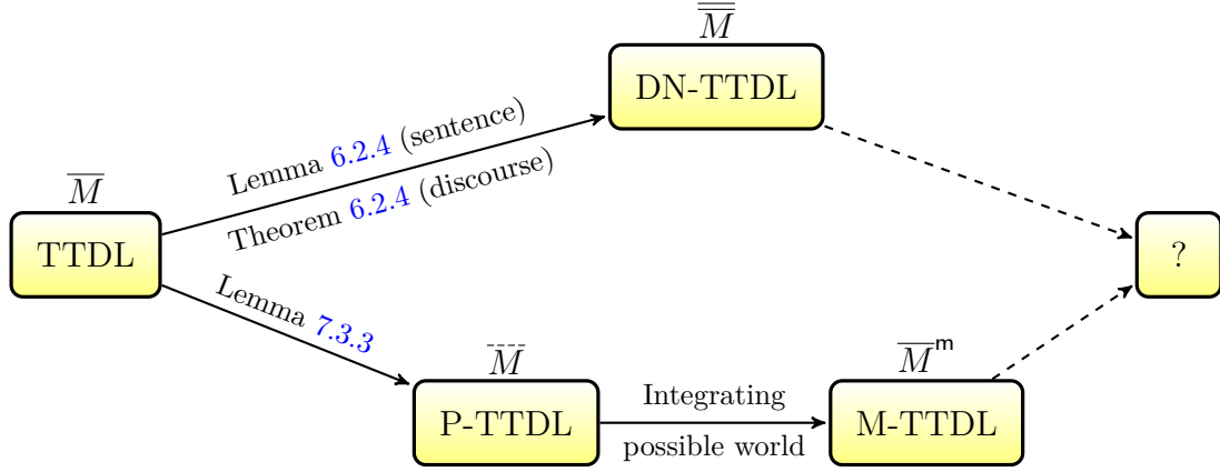
Fig. 7.11 Relations between All Frameworks
