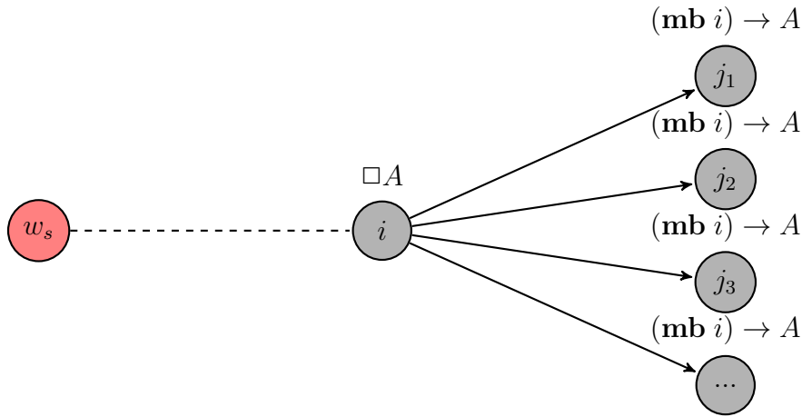
Fig. 7.3 Possible Worlds Hierarchy of \Box A
