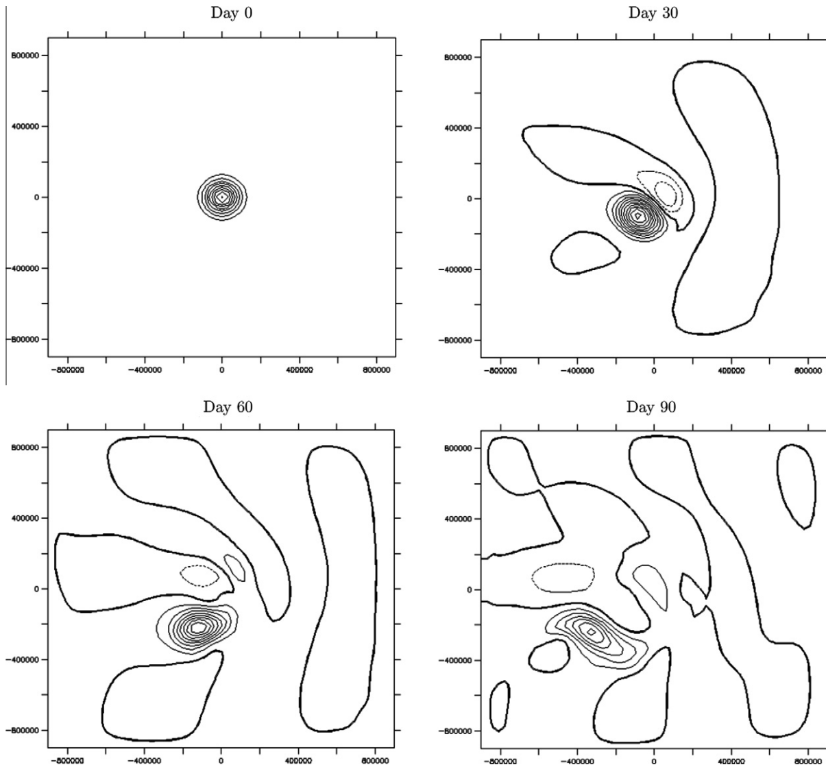
Fig. 12. Evolution of surface elevation in the coarse, non-nested, solution. The contour interval is 10 cm.
