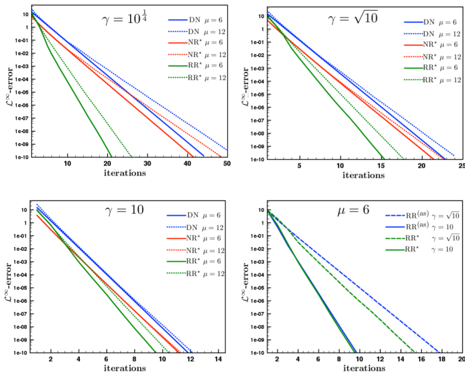
Figure 2.5: Convergence for \gamma = 10^{\frac{1}{4}} (top, left), \gamma = \sqrt{10} (top, right) and \gamma = 10 (bottom, left) for \mu = 6 and \mu = 12 in the DN, RR*, and NR* cases. Comparison between RR* and RR (as) (bottom, right)
