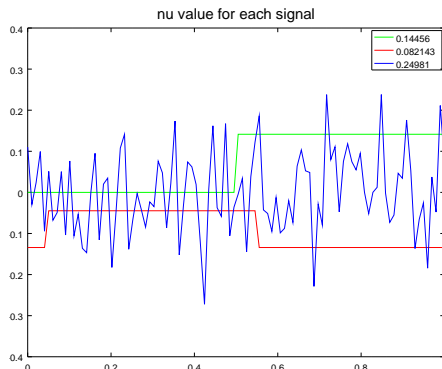
Figure 3.8: Different signals and their \theta(t_0) approximated with a sample of size 10^3 in \mathbb{R}^{\mathbb{Z}/100\mathbb{Z}} . \varepsilon is here a Gaussian noise in \mathbb{R}^{\mathbb{Z}/100\mathbb{Z}} , such that \mathbb{E}(\varepsilon) = 0 and \mathbb{E}(\|\varepsilon\|^2) = 1 . For instance the blue signal is a signal defined randomly, and when we approximate the \theta(t_0) which corresponds to that t_0 we find \simeq 0.25 .
