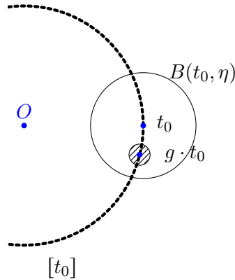
Figure 3.6: The smallest disk is included in the support of X and the points in that disk is closer from g \cdot t_0 than from t_0 . According to theorem 3.4 there is an inconsistency.
