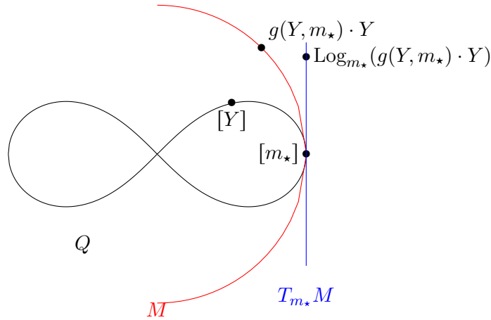
Figure 5.2: Representation of the quotient, M acts as an intermediary between the quotient space and the tangent plan at m_\star . If m_\star is a minimizer of the pre-variance in the quotient space, then \mathbb{E}(\text{Log}_{m_\star}(\text{Qlog}_{m_\star})Y) = 0 . Where \text{Qlog}_{m_\star}(Y) is the registration of Y to m_\star and \text{Log}_{m_\star} is the Riemannian logarithm map.
