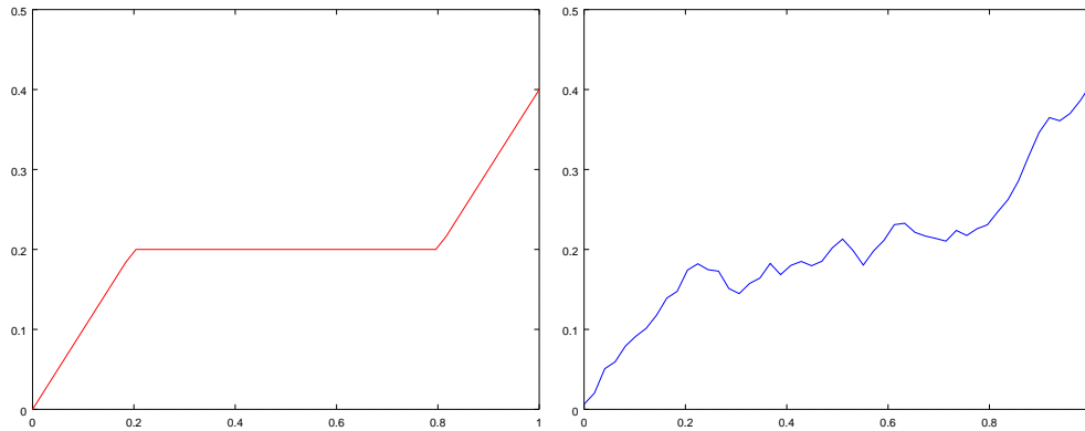
(a) The original template has a large isotropy: any bijective map which is equal to identity on (0, 0.2) \cup (0.8, 1) . (b) Due to the noise, there is no more bijective map which leaves invariant this noisy template.
