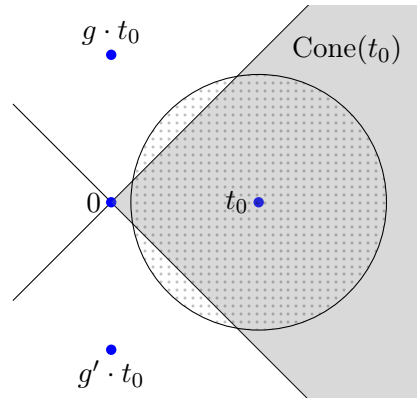
Figure 2.1: Planar representation of a part of the orbit of the template t_0 . The lines are the hyperplanes whose points are equally distant of two distinct elements of the orbit of t_0 , \text{Cone}(t_0) represented in points is the set of points closer from t_0 than any other points in the orbit of t_0 . Theorem 2.1 states that if the support (the dotted disk) of the random variable X is not included in this cone, then there is an inconsistency.
