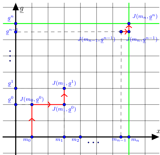
Figure 3.3: Iterative minimization of the function J on the two axes, the horizontal axis represents the variable in the space M , the vertical axis represents the set of all the possible registrations G^I . Once the convergence is reached, the point (m_n, g_n) is the minimum of the function J on the two axis in green. Is this point the minimum of J on its whole domain? There are two pitfalls: firstly this point could be a saddle point, it can be avoided with proposition 3.3, secondly this point could be a local (but not global) minimum, this is discussed in section 3.2.4.3
