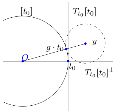
Figure 2.7: y \notin T_{t_0}[t_0]^\perp therefore y is closer from g \cdot t_0 for some g \in G than t_0 itself. In conclusion, if y is in the support of X , there is an inconsistency.
