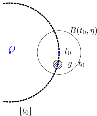
Figure 2.6: The smallest disk is included in the support of X and the points in that disk is closer from g \cdot t_0 than from t_0 . According to theorem 2.4 there is an inconsistency.
