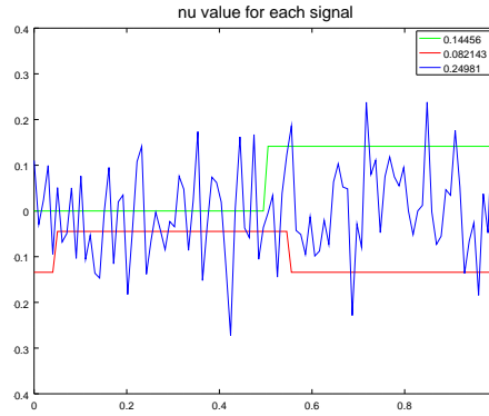
Figure 2.8: Different signals and their \theta(t_0) approximated with a sample of size 10^3 in \mathbb{R}^{\mathbb{Z}/100\mathbb{Z}} . \varepsilon is here a Gaussian noise in \mathbb{R}^{\mathbb{Z}/100\mathbb{Z}} , such that \mathbb{E}(\varepsilon) = 0 and \mathbb{E}(\|\varepsilon\|^2) = 1 . For instance the blue signal is a signal defined randomly, and when we approximate the \theta(t_0) which corresponds to that t_0 we find \simeq 0.25 .
