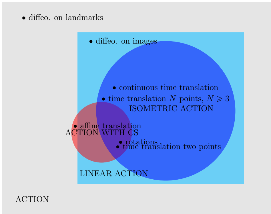
Figure 5.1: Different kind of actions according to their property, the actions in bullet are examples of each cases. The definition and the existence of such congruent section (CS) was discussed in section 4.4.1, isometric actions were studied in chapters 2 and 3, linear actions in section 3.3.4. The examples of the diffeomorphism on landmarks or images were described in section 1.3.3, the affine translation in example 3.6, the time translation on two points in section 2.3.6, the time translation on more than two points in examples 2.1 and 4.2, the continuous time translation in examples 2.3 and 4.3, rotations in section 2.4.6.3 and example 4.1
