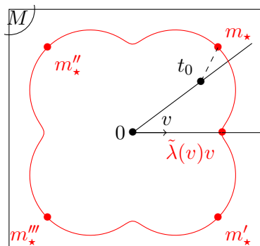
Figure 3.2: We minimize the variance on each half-line \mathbb{R}^+v where \|v\| = 1 . The element which minimizes the variance on such a half-line is \tilde{\lambda}(v)v , where \tilde{\lambda}(v) \geq 0 . We get a surface in M by S \in v \mapsto \tilde{\lambda}(v)v (which is a curve in this figure since we draw it in dimension 2). The proof of theorem 3.1 states that if [m_\star] is a Fréchet mean then m_\star is an extreme point of this surface. On this picture there is 4 extreme points which are in the same orbit: we took here the simple example of the group of rotations of 0, 90, 180 and 270 degrees.
