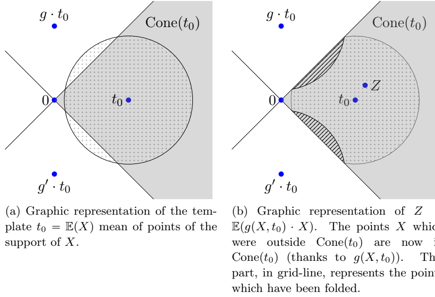
Figure 2.2: Z is the mean of points in \text{Cone}(t_0) where \text{Cone}(t_0) is the set of points closer from t_0 than g \cdot t_0 for g \in G \setminus e_G . Therefore it seems that Z is higher than t_0 , therefore \nabla F(t_0) = 2(t_0 - Z) \neq 0 .
