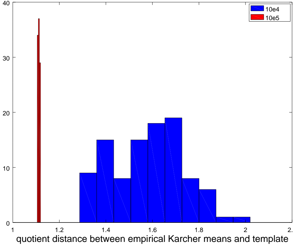
Figure 3.8: Histogram of the quotient distance between the template and the output of the max-max algorithm, in red we have the distribution of the distance of 100 max-max algorithm with the same sample of size 10^5 , in blue the distribution with a sample of size 10^4 . The larger the size of the sample, the more concentrated the distance is.
