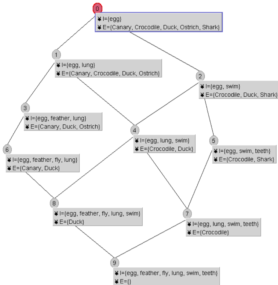
Figure 2.4: Concept lattice constructed from the formal context introduced in Table 2.5. Each node is a formal concept composed of its extent (set of objects) and its intent (set of attributes).
