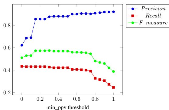
Figure 4.10: The effect of quality threshold on precision , recall and F-Measure values.
