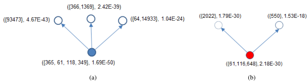
Figure 6.7: Two examples of (a) selected and (b) discarded concepts from the lattice.
