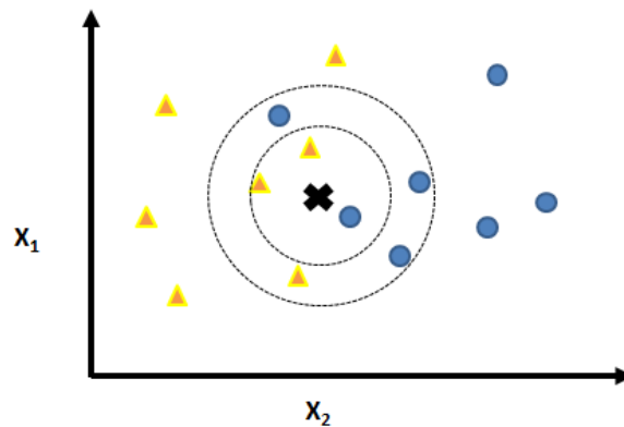
Figure 2.2: Two examples of k-NN classification in two dimensions. The test instance (black cross) should be classified either to the blue circle class or to the yellow triangle class. If k = 3 , it is assigned to the yellow triangle class because there are 2 yellow triangles and only 1 blue circles inside the inner dashed circle. If k = 7 , it is assigned to the blue circle class because there are 4 blue circles vs. 3 yellow triangles inside the outer dashed circle.
