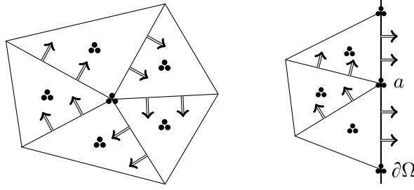
Figure 2.4 – The degrees of freedom of the space \underline{\underline{\Sigma}}_h^a in the case m = 1 on a patch for a \in \mathcal{V}_h^{\text{int}} (left) and a \in \mathcal{V}_h^{\text{ext}} (right)
