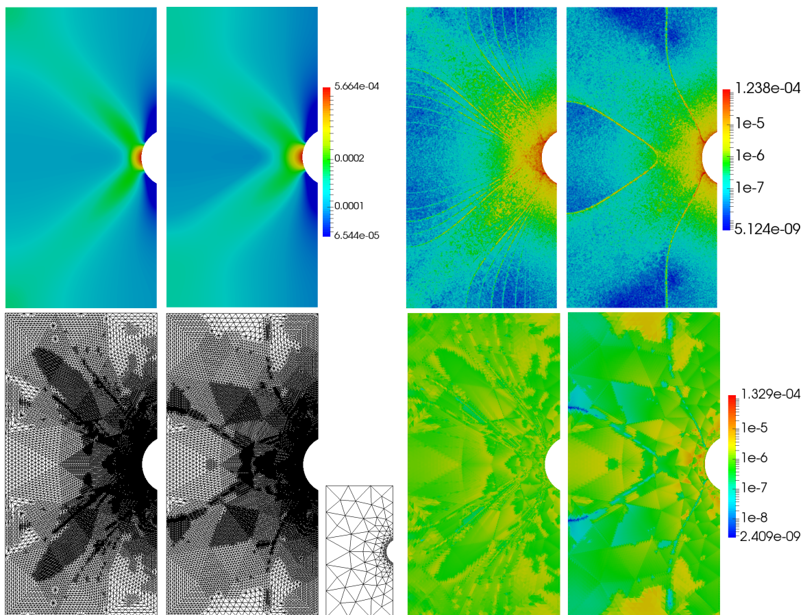
Figure 3.6 – Notched specimen plate, comparison between Hencky–Mises (left in each picture) and damage model (right). Top left: \text{tr}(\nabla_s \underline{u}_h) . Top right: \eta_{\text{disc}} on a fine mesh (no adaptive refinement). Bottom left: meshes after six adaptive refinements. Bottom middle: initial mesh. Bottom right: \eta_{\text{disc}} on the adaptively refined meshes.
