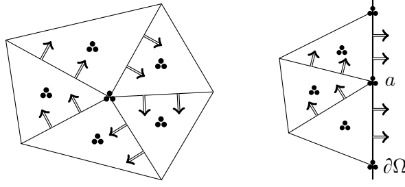
Figure 2.4 – The degrees of freedom of the space \underline{\Sigma}_h^a in the case m = 1 on a patch for a \in \mathcal{V}_h^{\text{int}} (left) and a \in \mathcal{V}_h^{\text{ext}} (right)
