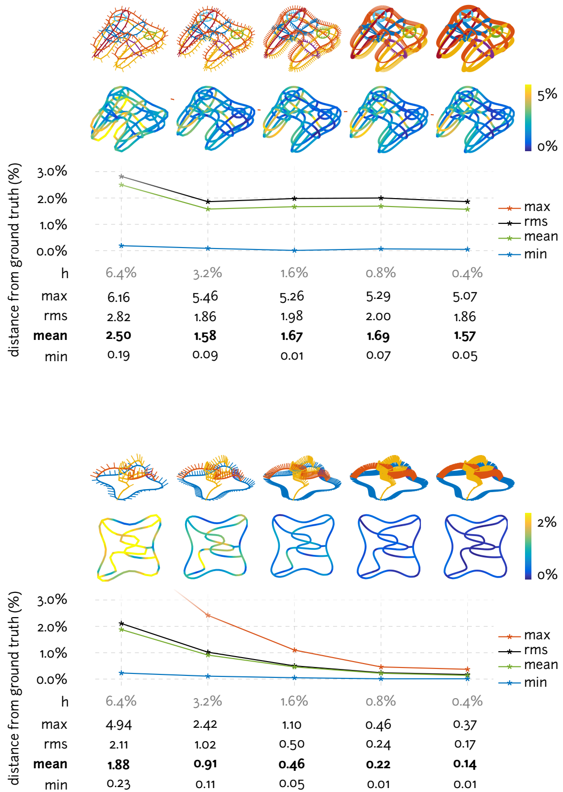
Figure 3.17: Network error, gamepad &amp; lilium, synthetic
