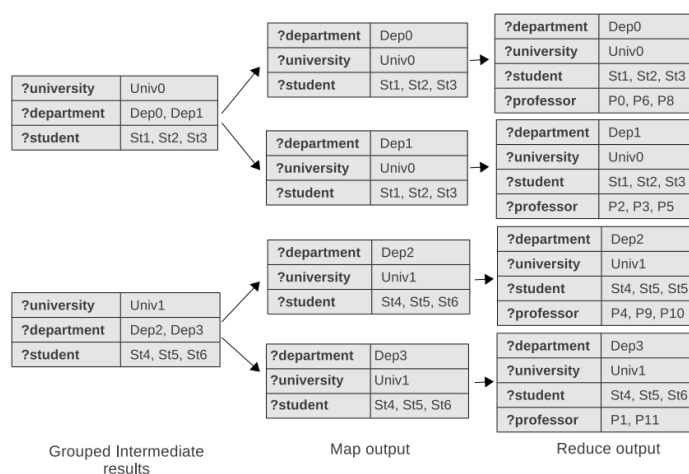
Figure 7.3: Join on grouped intermediate results [Papailiou et al., 2013]
