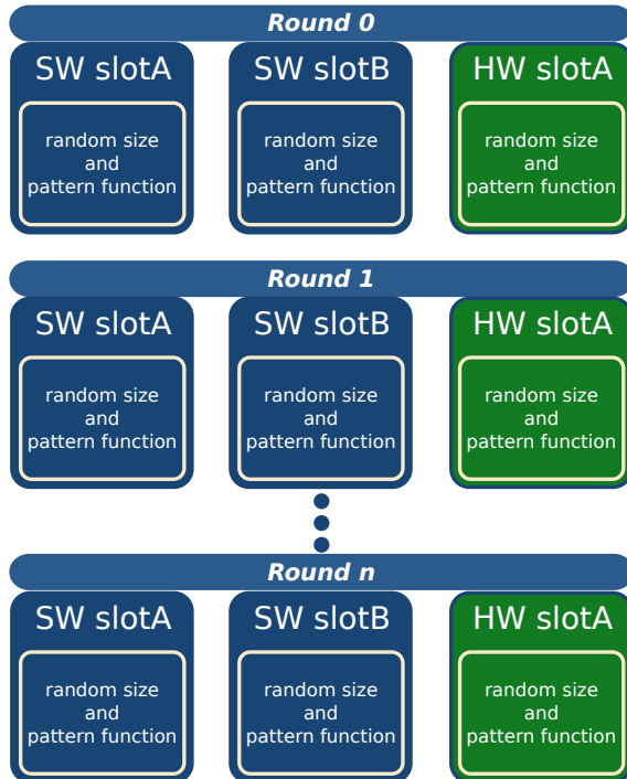
Figure 4-17 – Overview of a mutant application structure.
