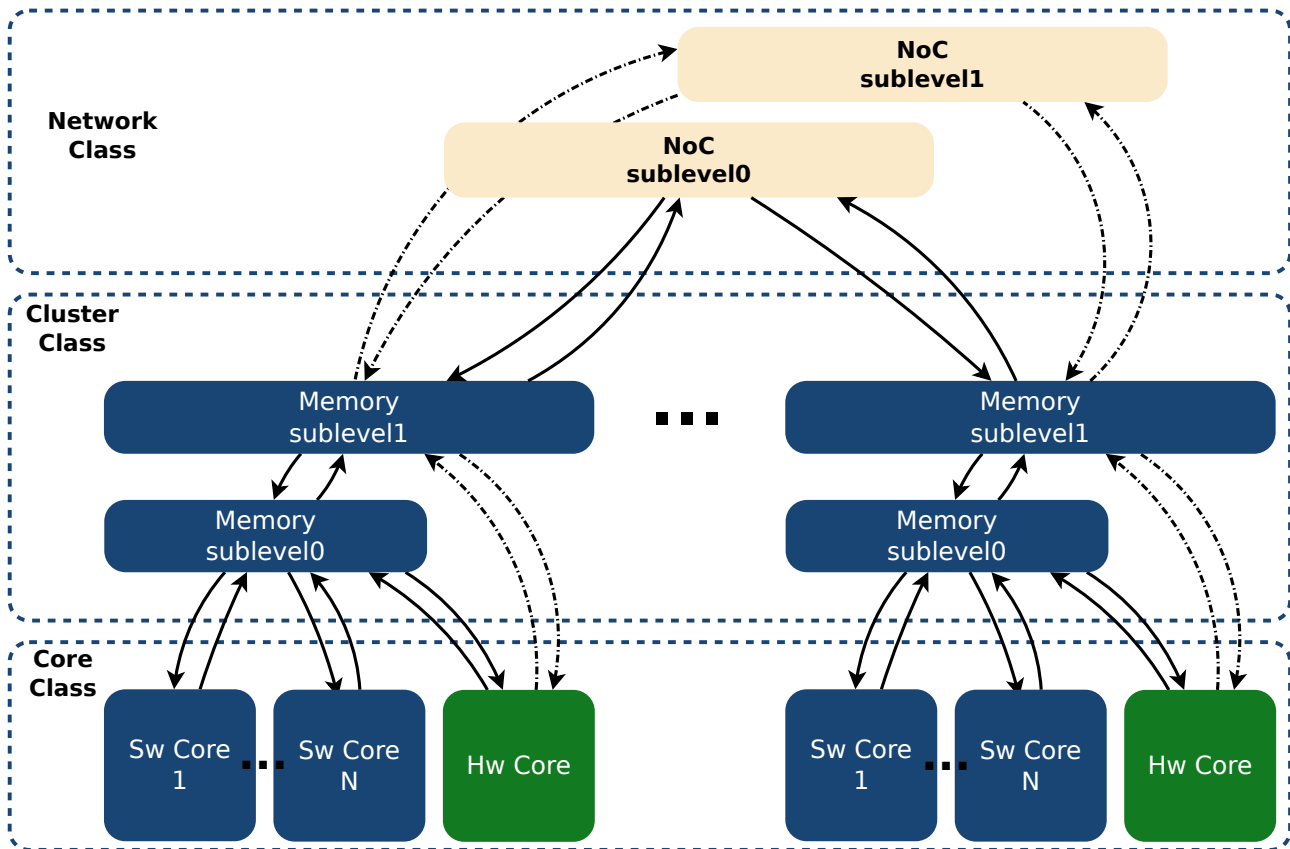
Figure 2-10 – Oriented-tree memory hierarchies abstraction.
