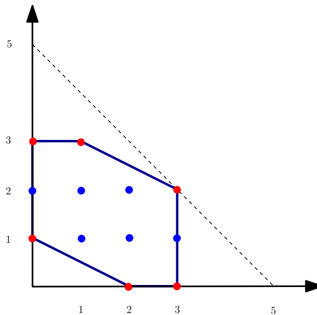
Figure 4.6: The discriminant polytope
