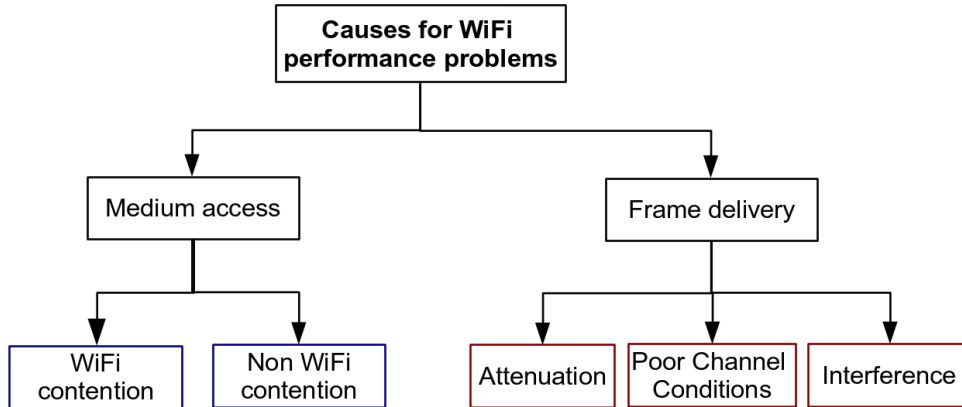
Figure 1.4: Causes of Wi-Fi performance problems
