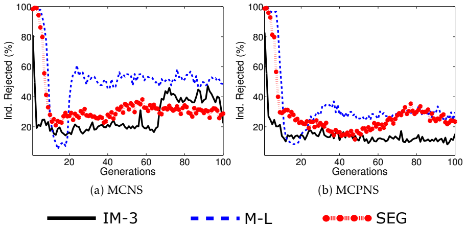
Figure 9.9: Plot showing the percentage of rejected individuals, with respect to the population size, that did not satisfy the MC.
