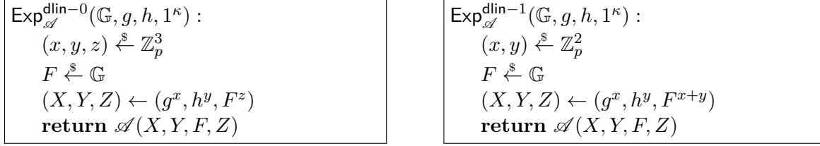
Figure 2.5: Experiments \text{Exp}_{\mathcal{A}}^{\text{dlin}^{-0}}(\mathbb{G}, g, h, 1^\kappa) and \text{Exp}_{\mathcal{A}}^{\text{dlin}^{-1}}(\mathbb{G}, g, h, 1^\kappa) for the decision linear assumption over a group \mathbb{G} with generators (g, h)
