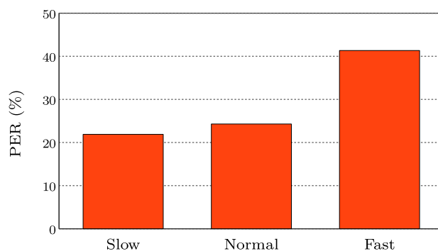
Figure 3.2: PER (%) between canonical and realized phonemes in words with fast, normal and slow speaking rates. Speaking rate is calculated by dividing the number of syllables in a word by its duration. All speaking rates are then binned into three categories with equal probability masses.
