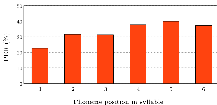
Figure 3.8: PER (%) with respect to position of phonemes in syllable.
