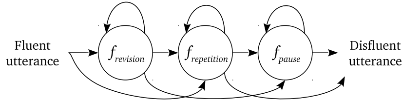
Figure 5.1: Complete process of disfluency generation.
