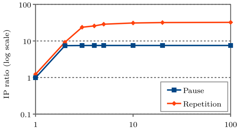
Figure 5.8: Correlation between number of hypotheses and IP ratio.
