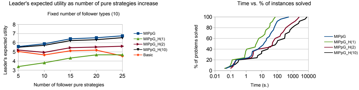
Figure 5.6.1: Quality of the lower bound and solution time using (MIPpG_H)
