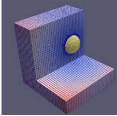
Octrees Mesh Refinement (Optimad, Triangular mesh refinement (Noureddine Hannoun c )
