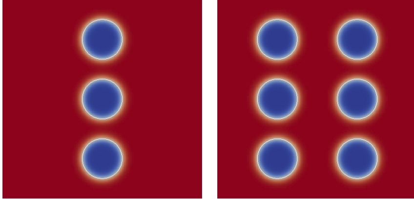
Figure 5.12: Conductivity term (\kappa_G, \kappa_S) = (40, 0.514) \text{ Wm}^{-1}K^{-1} .
