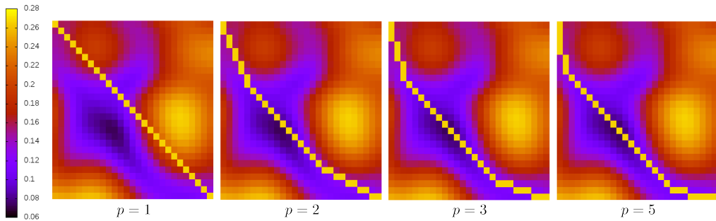
Figure 2.13 – Examples of a dynamic time warping path with various slope constraints
