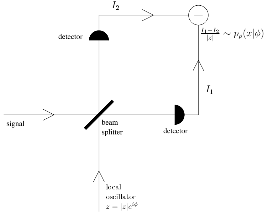
Figure 2.2: Quantum Homodyne Tomography measurement set-up
