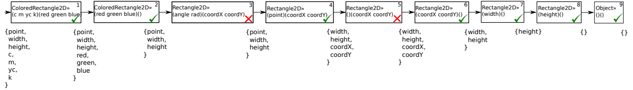
Figure 2.9: Execution flow of the object creation.
