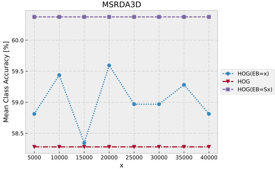
Figure 5.6: Results on MSRDA3D dataset. The plot shows Mean Class Accuracy for HOG normalized with different EB values (blue dotted line). The standard HOG performance is showed in red, while EB=s_x is shown in purple. The figure shows that HOG all tested EB values as well as EB=s_x outperform standard HOG descriptor. The EB=s_x for MSRDA3D is equal to 7696.
