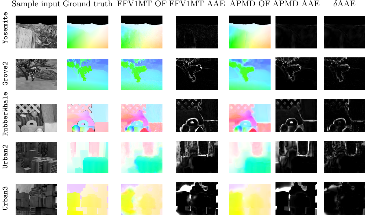
Figure 4.4: Sample results on Yosemite sequence and a subset of Middlebury training set. \delta AAE = AAE_{FFV1MT} - AAE_{APMD}
