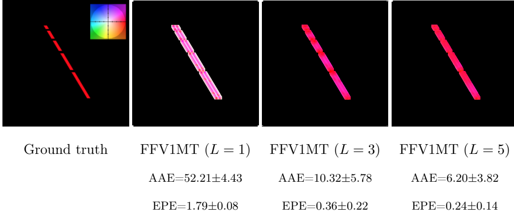
Figure 3.6: Influence of the number of spatial scales. The FFV1MT model is tested with L=1 , 3 and 5 scales. The color code used to show optical flow is in the inset on the first image. This color code will be used in all figures to represent optical flow. Note that the aperture problem is partially solved by considering a scale-space approach, where the effective receptive field size of MT increases and thus takes into consideration 2-D cues that are present at a distance. This can be readily observed by the results on bars with different lengths.
