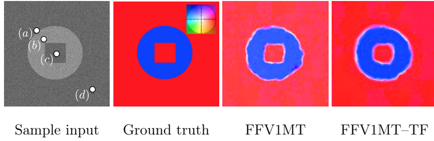
Figure 3.7: Results on a synthetic video: A translating shape is moving with velocity v = (-3, -3) ppf on top of a translating background moving with velocity v = (4, 0) ppf. Results are \text{AAE}=3.56\pm 14.40 , \text{EPE}=0.26\pm 0.86 for FFV1MT and \text{AAE}=3.70\pm 14.78 , \text{EPE}=0.27\pm 0.86 for FFV1MT-TF.
