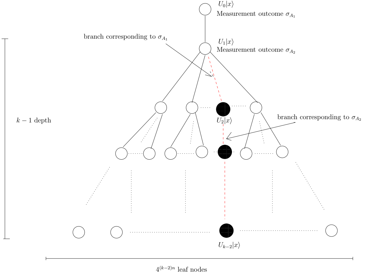
Figure 3.1: Pictorial view of Step 3 of Algorithm 1: Each level of the tree corresponds to a round trip between Alice and Bob. Each of the nodes correspond to a quantum state. In particular, the root node is the initial quantum state U_0|x\rangle received by Alice, and the path in red dash (determined by the successive outputs of the Bell measurements) goes along the various states held by Alice at different steps of the protocol, namely U_1|x\rangle, \dots, U_{k-2}|x\rangle .
