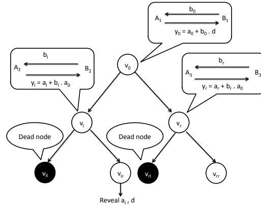
Figure 5.1: Pictorial view for an internal node of the Tree protocol. Here the coloring is such that c(v) = 1, c(vl) = 2, c(vr) = 3 .
