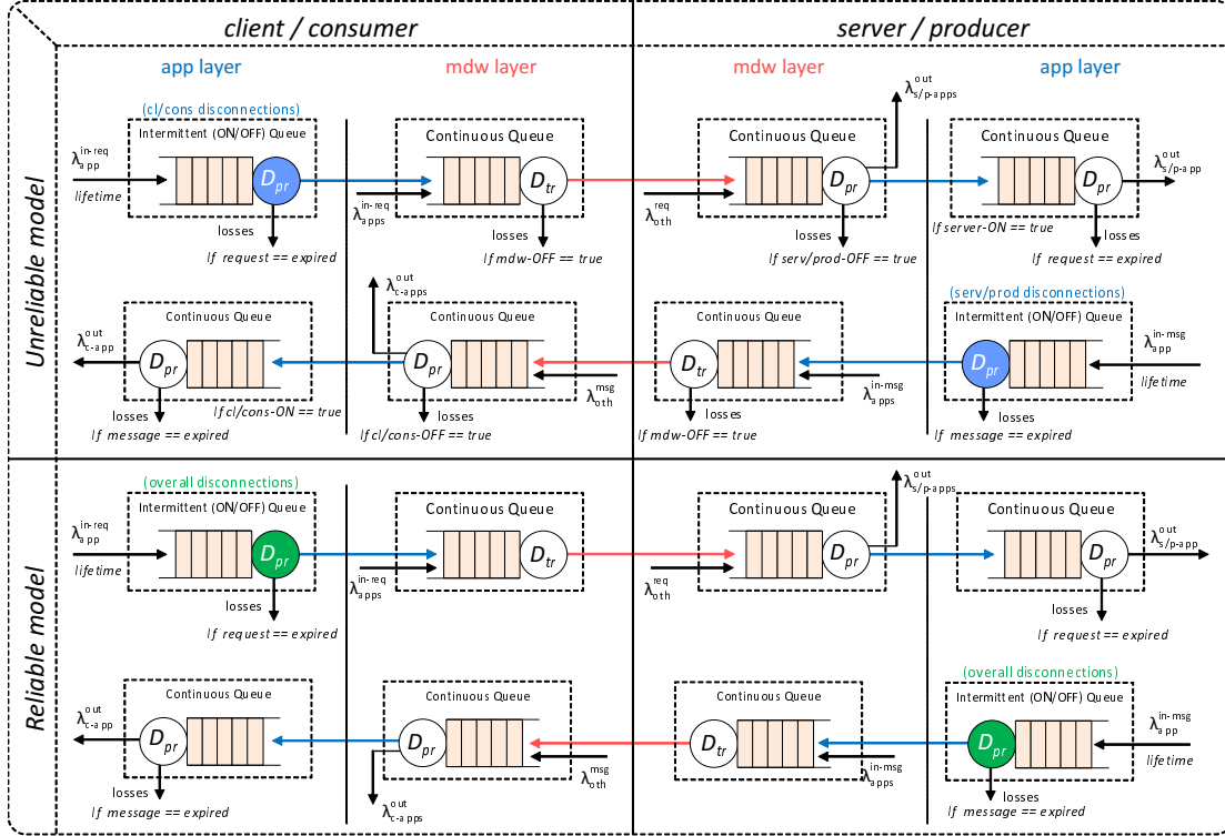
Figure 5.9: PerfMP for CS two-way async/stream interactions.
