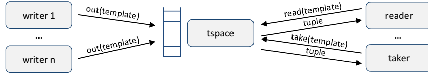
Figure 3.9: TS semantics.
