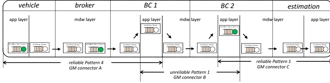
Figure 5.14: End-to-end queuing network for the vehicle-device \rightarrow estimation-service interconnection.
