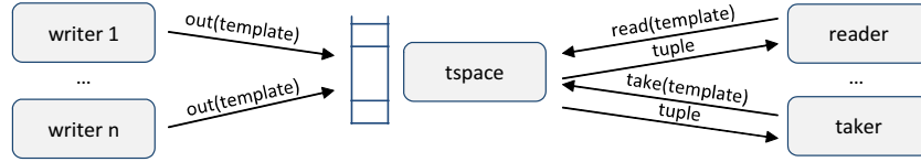
Figure 3.9: TS semantics.
