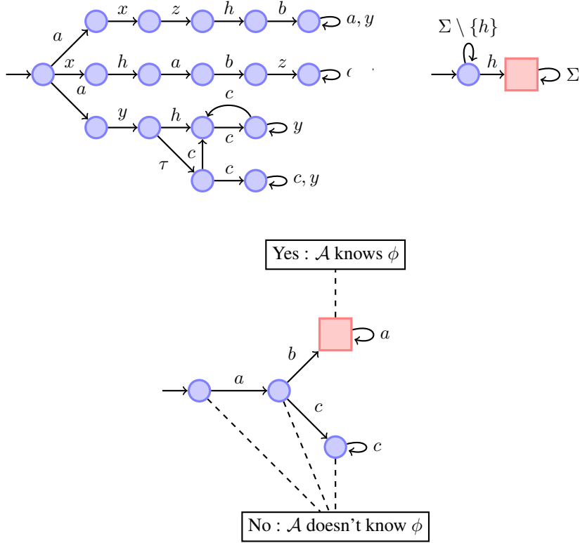
Figure 4.6: \mathcal{G} , \mathcal{A}_\varphi and the corresponding \mathcal{O}_A^\varphi
