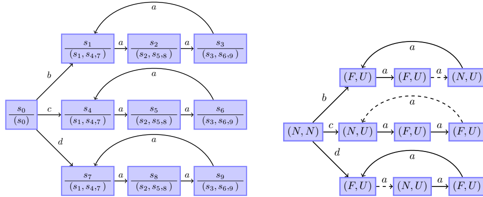
Figure 2.24: \mathcal{A} = \mathcal{G} \times \text{Det}_{\Sigma_o}(\mathcal{G}) and its abstract view
