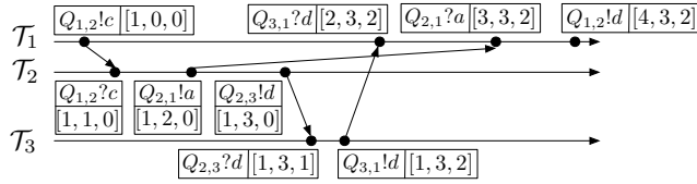
Figure 3.10: An execution of the running example.
