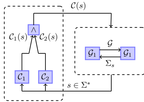
Figure 3.3: Supervision Scheme
