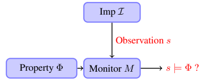
Figure 3: Run-time Verification principle
