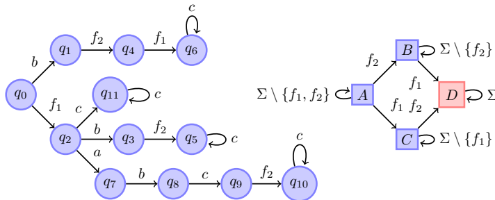
Figure 2.11: LTS \mathcal{G}_1
