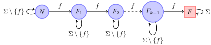
Figure 2.4: k occurrences of the same fault f
