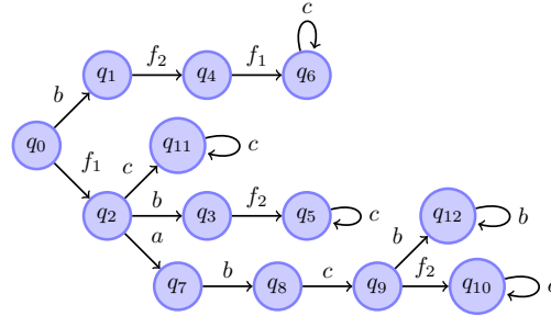
Figure 2.13: LTS \mathcal{G}_2
