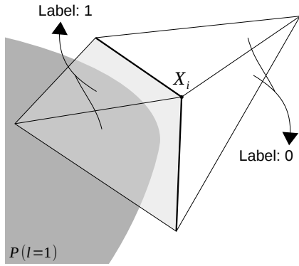
(a) Initial configuration around X_i .
