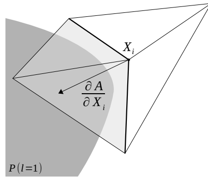
(d) The summation of the vectors in (c) yields an estimation of the gradient.
