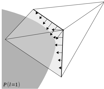
(c) Resulting vectors \eta(u)\lambda_i(u)\hat{n}(u) (scaled by the shape function \lambda_i , see Eq. 6.6).
