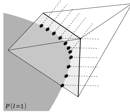
(b) Ray shooting from various points u normal to the edges to estimate relative orientations \eta(u) .
