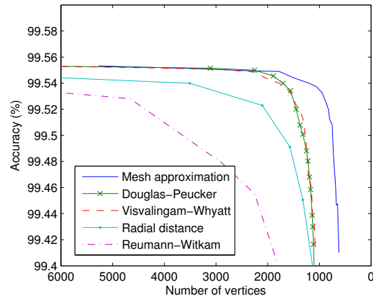
Figure 6.7: Performance comparison.
