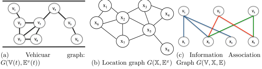
Figure 3.1: Network Model
