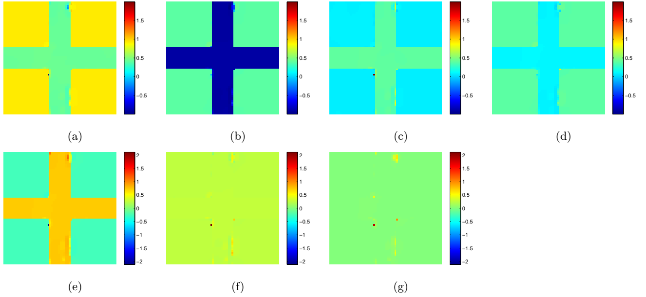
Figure 4.16: Estimation of Gradient Descent method with projection, initial guess u_{01} = (1, i0) . (a) \text{Re}\{\hat{u}\} , (b) \text{Im}\{\hat{u}\} , (c) |\text{Re}\{\hat{u}\} - \text{Re}\{\check{u}\}| , (d) |\text{Im}\{\hat{u}\} - \text{Im}\{\check{u}\}| , (e) \hat{\phi} , (f) |\hat{\phi} - \check{\phi}| , (g) |\check{\phi}_j - \hat{\phi}_j - \check{\phi} - \hat{\phi}|
