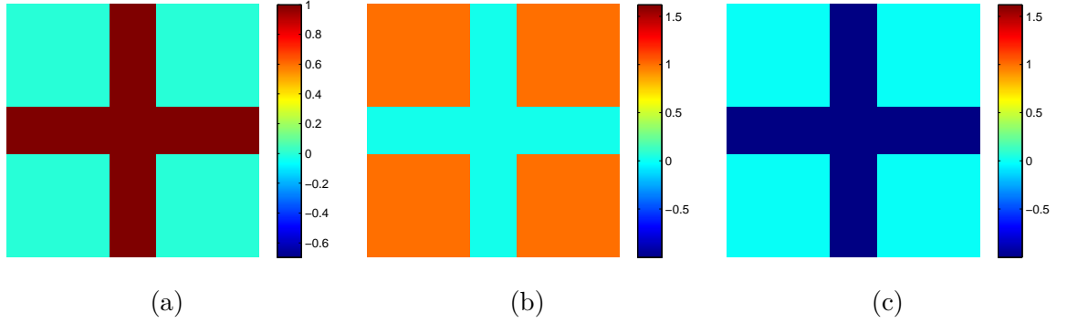
Figure D.19: Cross object. True values for phase and specimen functions (a) Phase function \check{\phi} , (b) \text{Re}\{\tilde{u}\} , (c) \text{Im}\{\tilde{u}\}
