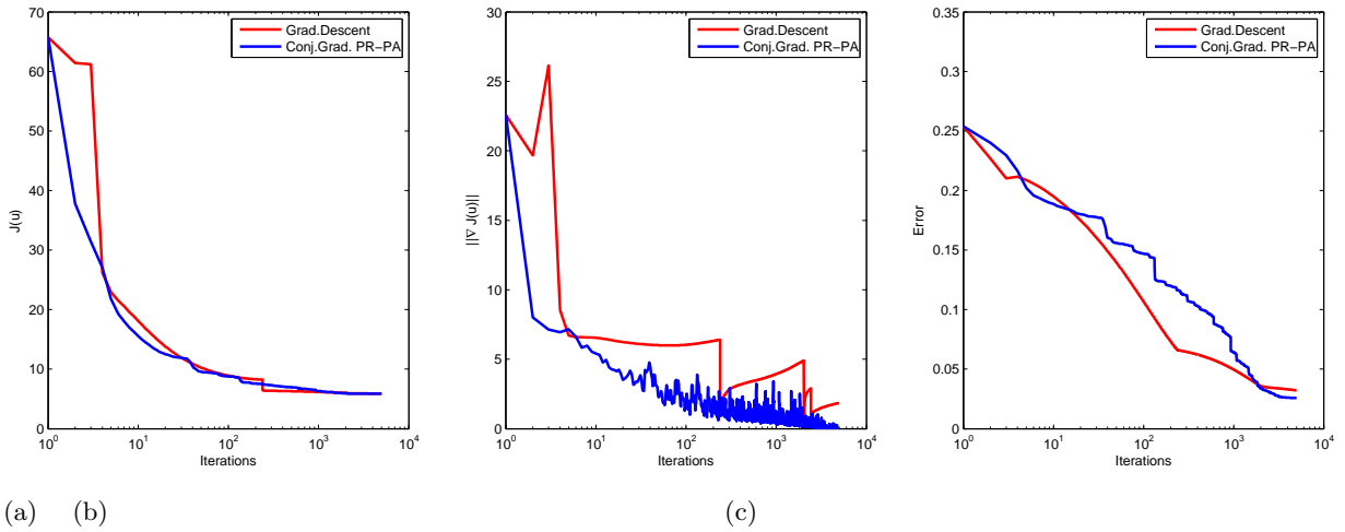
Figure 4.6: Methods comparison without projection, initial guess u_{01} = (1, i0) . (a) Convergence, (b) Norm of gradient, (c) Error
