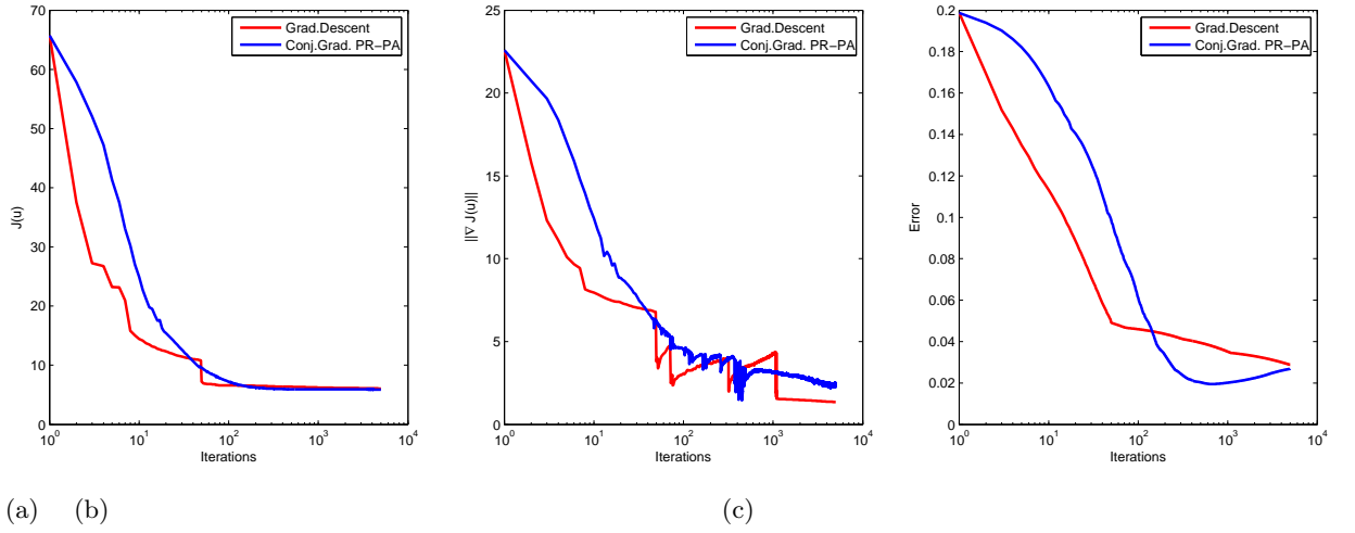
Figure D.10: Methods comparison with projection, initial guess u_{02} = \left(\frac{1}{\sqrt{2}}, i\frac{1}{\sqrt{2}}\right) . (a) Convergence, (b) Norm of gradient, (c) Error
