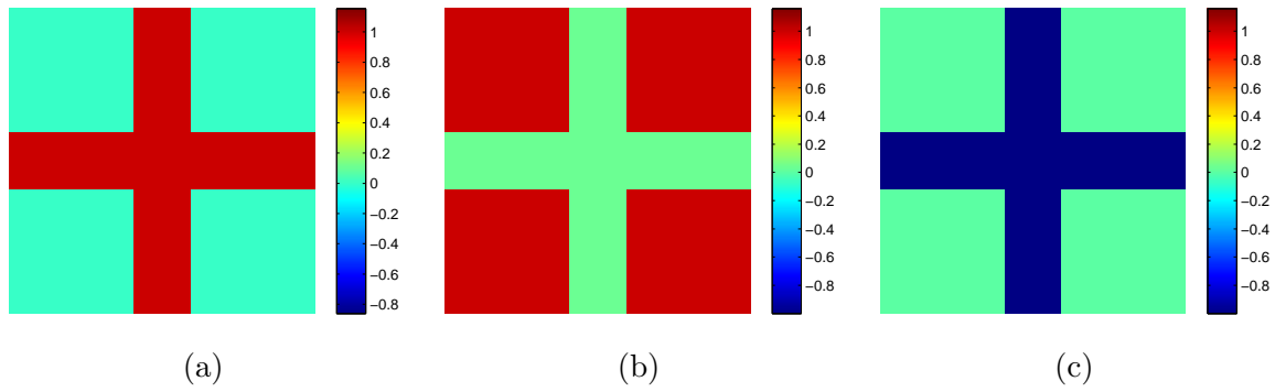
Figure D.17: Cross object. True values for phase and specimen functions (a) Phase function \check{\phi} , (b) \Re \{\check{u}\} , (c) \Im \{\check{u}\}
