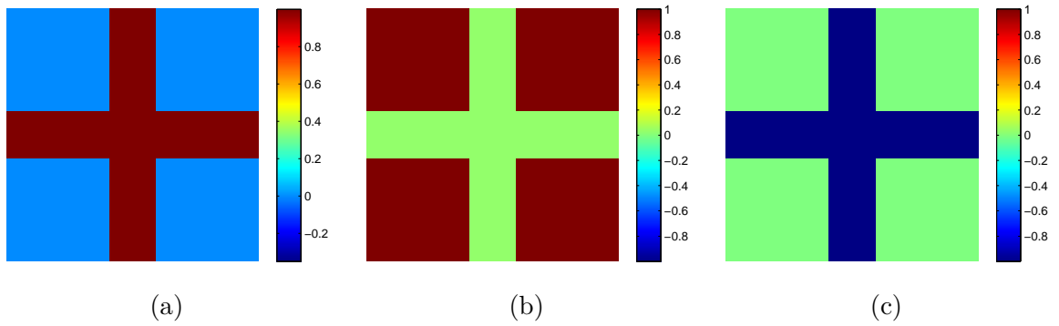
Figure D.11: Cross object. True values for phase and specimen functions (a) Phase function \check{\phi} , (b) \Re\{\check{u}\} , (c) \Im\{\check{u}\}
