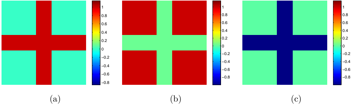
Figure 4.19: Cross object. True values for phase and specimen functions (a) Phase function \check{\phi} , (b) \Re\{\check{u}\} , (c) \Im\{\check{u}\}
