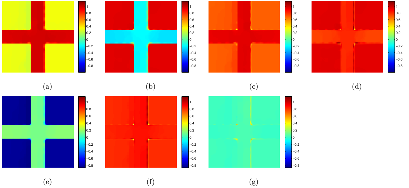
Figure 4.20: Estimation of Gradient Descent method without projection, initial guess u_{02} = (\frac{1}{\sqrt{2}}, i\frac{1}{\sqrt{2}}) . (a) \Re\{\hat{u}\} , (b) \Im\{\hat{u}\} , (c) |\Re\{\hat{u}\} - \Re\{\check{u}\}| , (d) |\Im\{\hat{u}\} - \Im\{\check{u}\}| , (e) \hat{\phi} , (f) |\hat{\phi} - \check{\phi}| , (g) |\check{\phi}_j - \hat{\phi}_j - \overline{\check{\phi} - \hat{\phi}}|
