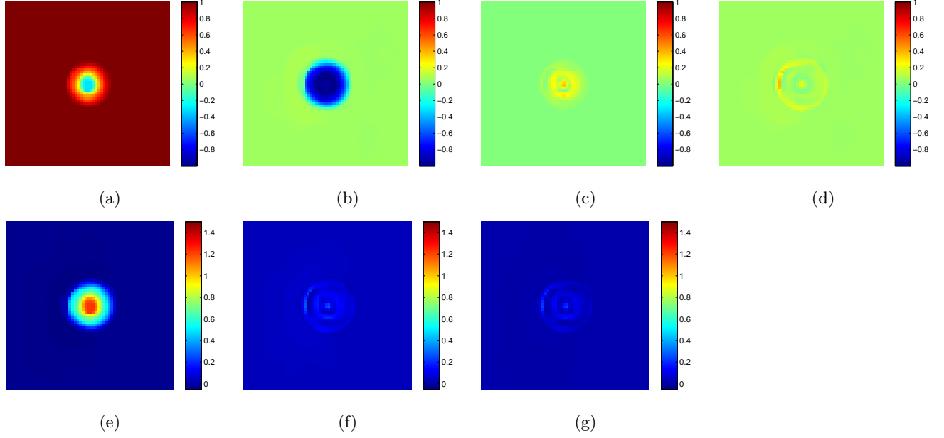
Figure 4.5: Estimation of Gradient Descent method with projection, initial guess u_{01} = (1, i0) . (a) \text{Re}\{\hat{u}\} , (b) \text{Im}\{\hat{u}\} , (c) |\text{Re}\{\hat{u}\} - \text{Re}\{\tilde{u}\}| , (d) |\text{Im}\{\hat{u}\} - \text{Im}\{\tilde{u}\}| , (e) \hat{\phi} , (f) |\hat{\phi} - \check{\phi}| , (g) |\check{\phi}_j - \hat{\phi}_j - \check{\phi} - \hat{\phi}|
