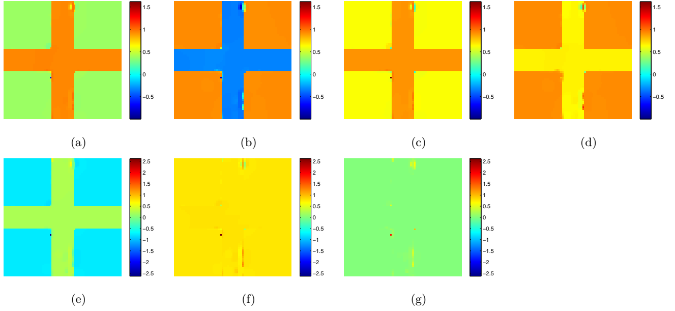
Figure 4.22: Estimation of Gradient Descent method with projection, initial guess u_{02} = (\frac{1}{\sqrt{2}}, i\frac{1}{\sqrt{2}}) . (a) \text{Re}\{\hat{u}\} , (b) \text{Im}\{\hat{u}\} , (c) |\text{Re}\{\hat{u}\} - \text{Re}\{\check{u}\}| , (d) |\text{Im}\{\hat{u}\} - \text{Im}\{\check{u}\}| , (e) \hat{\phi} , (f) |\hat{\phi} - \check{\phi}| , (g) |\check{\phi}_j - \hat{\phi}_j - \check{\phi} - \hat{\phi}|
