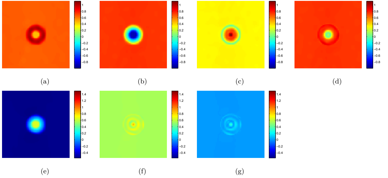
Figure 4.9: Estimation of Gradient Descent method without projection, initial guess u_{02} = \left(\frac{1}{\sqrt{2}}, i\frac{1}{\sqrt{2}}\right) . (a) \text{Re}\{\hat{u}\} , (b) \text{Im}\{\hat{u}\} , (c) |\text{Re}\{\hat{u}\} - \text{Re}\{\check{u}\}| , (d) |\text{Im}\{\hat{u}\} - \text{Im}\{\check{u}\}| , (e) \hat{\phi} , (f) |\hat{\phi} - \check{\phi}| , (g) |\check{\phi}_j - \hat{\phi}_j - \overline{\check{\phi} - \hat{\phi}}|
