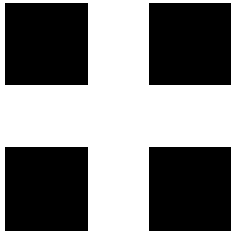
Figure 2.26: Simulated true phase object
