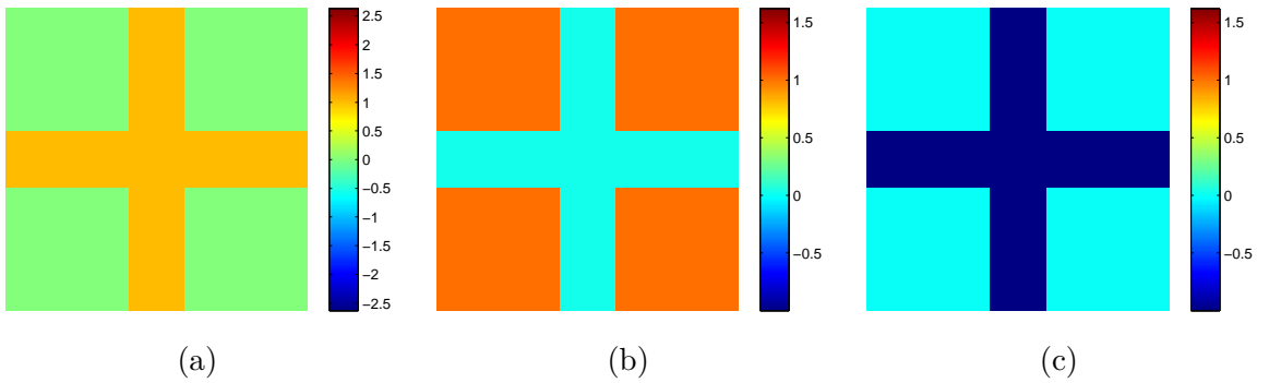
Figure 4.21: Cross object. True values for phase and specimen functions (a) Phase function \check{\phi} , (b) \Re\{\check{u}\} , (c) \Im\{\check{u}\}
