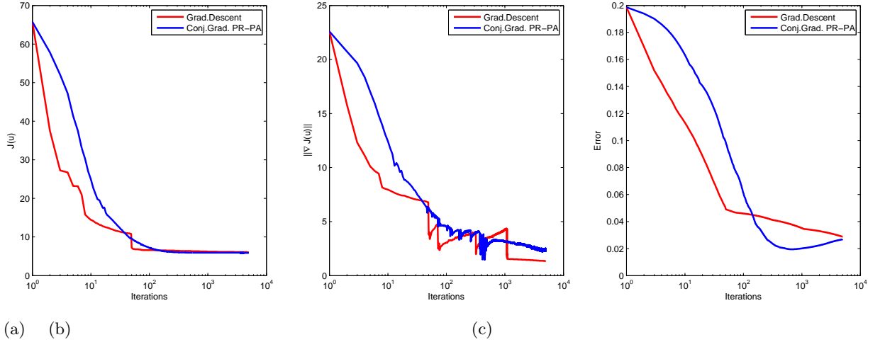
Figure 4.12: Methods comparison with projection, initial guess u_{02} = \left(\frac{1}{\sqrt{2}}, i\frac{1}{\sqrt{2}}\right) . (a) Convergence, (b) Norm of gradient, (c) Error
