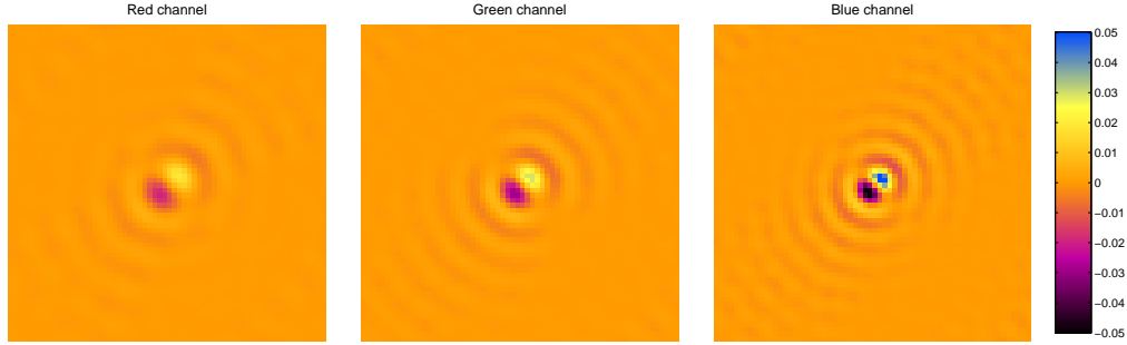
(b) \text{Real}\{h_{2,\lambda_\ell}(x,y)\}; \tau_2 = \pi/4
