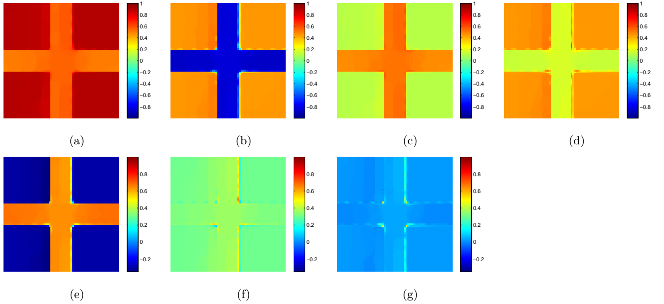
Figure 4.14: Estimation of Gradient Descent method without projection, initial guess u_{01} = (1, i0) . (a) \Re\{\hat{u}\} , (b) \Im\{\hat{u}\} , (c) |\Re\{\hat{u}\} - \Re\{\check{u}\}| , (d) |\Im\{\hat{u}\} - \Im\{\check{u}\}| , (e) \hat{\phi} , (f) |\hat{\phi} - \check{\phi}| , (g) |\check{\phi}_j - \hat{\phi}_j - \check{\phi} - \hat{\phi}|
