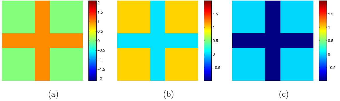
Figure 4.15: Cross object. True values for phase and specimen functions (a) Phase function \check{\phi} , (b) \text{Re}\{\check{u}\} , (c) \text{Im}\{\check{u}\}
