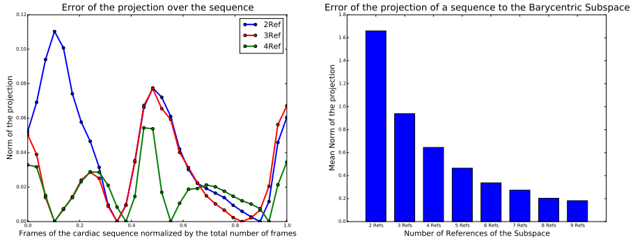
Figure 5.3: (Left): Example of the norm of the projection vector to the Subspace for 1 patient over the cardiac sequence with 1D , 2D and 3D –Barycentric Subspace. The projection is null for each of reference frames. (Right): Mean norm over all the frame of the sequences and averaged over all the patients for subspaces of increasing number of references/dimensionality.
