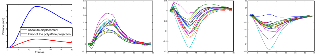
Figure 6.1: Polyaffine projection for a cardiac motion. (Left) figure: error of the projection versus absolute displacement. (Right) figures: diagonal parameters over time of the polyaffine matrix for each of the region of the left ventricle from which we can recognize (resp. from left to right) the radial, longitudinal and circumferential strains.
