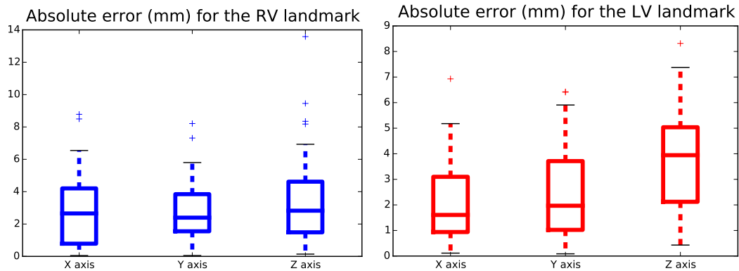
Figure 4.6: Absolute error on the test set for the detection of both landmarks along each axis. The error of the detection of the landmarks is comparable to the voxel spacing (on average 2.5\text{mm} \times 2.5\text{mm} \times 8\text{mm} for these images).
