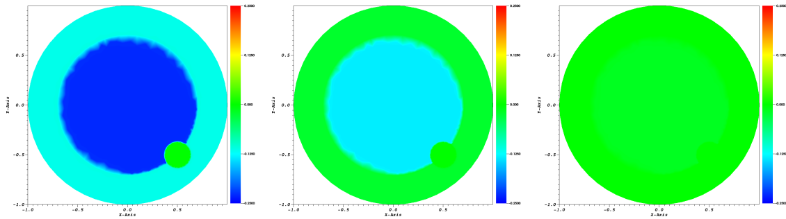
Figure 3.21: Triple point problem in Cartesian geometry. \frac{T_i - T_e}{T_e} 2-D fields at t = 2.1 \times 10^{-9} s (left), t = 4.7 \times 10^{-9} s (middle), and t = 1.35 \times 10^{-8} s (right).
