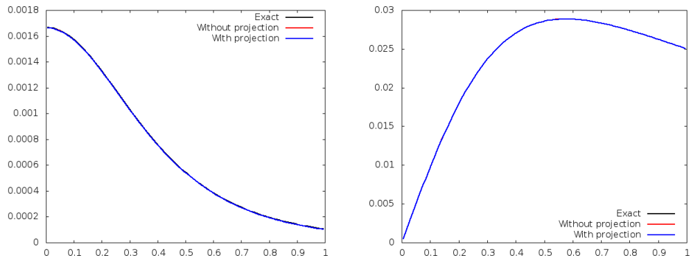
Figure 4.24: Screw pinch equilibrium in cylindrical coordinates, All R . HLLD O(1) . Left: Pressure, Right: B_\varphi .
