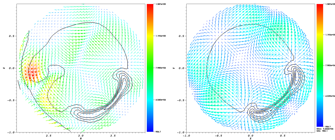
Figure 3.24: Triple point problem at t = 1.1574 \times 10^{-5}s . Comparison of the results obtained in Cartesian geometry and in a torus. Velocity vectors with density contours. Left: 2-D axisymmetric run, Right: 2-D Cartesian run.
