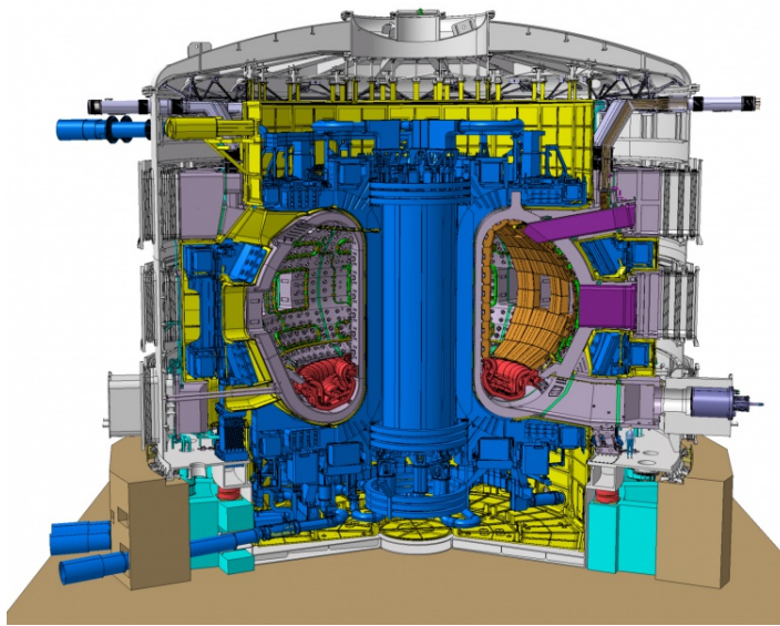
Figure 6: Representation of the future ITER tokamak [6].
