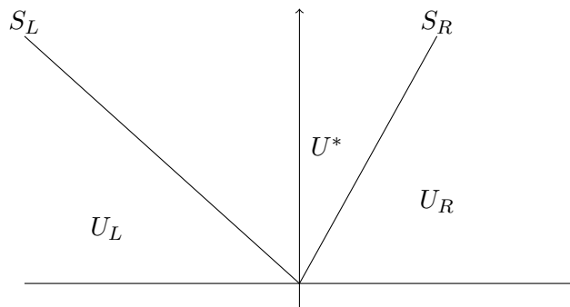
Figure 4.2: Riemann fan with one intermediate state.
