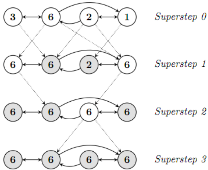
Figure 2.2 – Pregel model [12]
