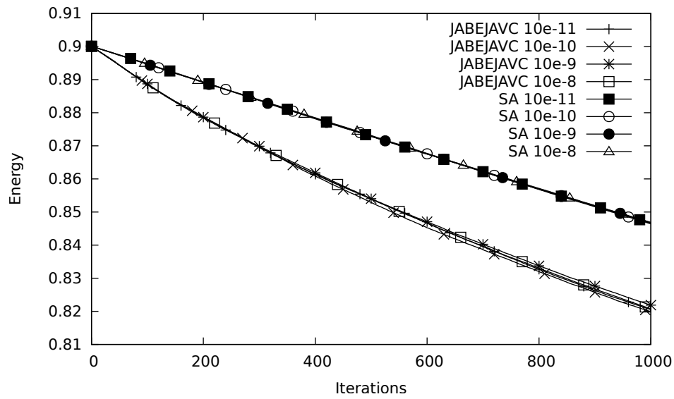
Figure 5.1 – \mathcal{E}_{comm} value for JA-BE-JA-VC and \mathcal{E} value for SA using email-Enron graph (1000 iterations were performed)
