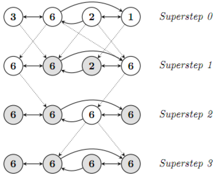
Figure 2.2 – Pregel model [12]
