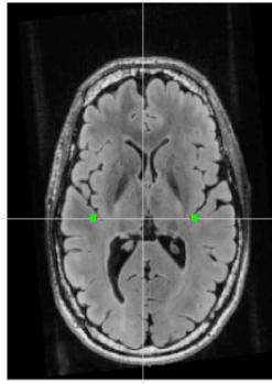
Figure 2.5: An example of dipole fitting. (source http://www.fielddtriptoolbox.org )
