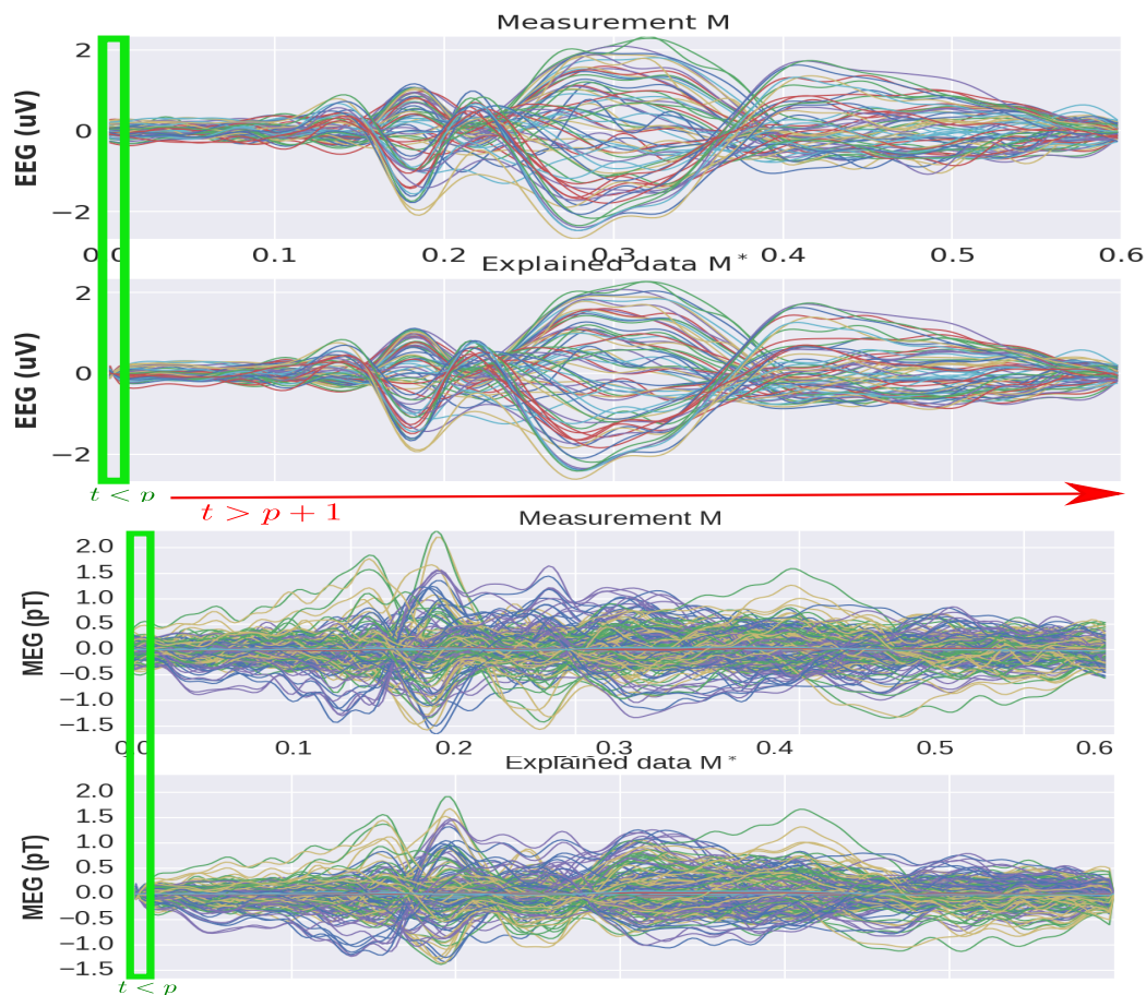
Figure 5.39: Acquired EEG and MEG data and the explained data, computed as G_d J_v , with iSDR(p = 2) of subject 15. We show the reconstructed MEG after magnitude debiasing. No magnitude debiasing is applied for reconstructed EEG. Our initialization favors small activations at the beginning, but could explain accurately the remaining time samples.
