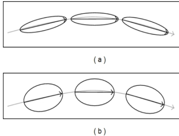
Figure 3.5: Schematic illustration of deterministic tractography, (a) three adjacent voxels have a clearly directed primary diffusion direction (longitudinal diffusion) indicated by ellipsoids. A deterministic tractography analysis would result in the indicated tract. (b) weak directionality of diffusion, evidenced by more spherical ellipsoids (small FA). The direction of the principal direction is, however, unchanged. This explains why deterministic tractography analysis may result in the same reconstructed tract (primary direction unchanged) although the diffusion tensor is less ellipsoidal. (Xekardaki et al., 2011)
