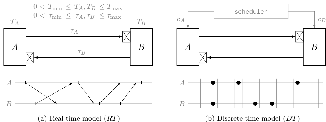
Figure 4.1: Soundness: A property \varphi true for the discrete-time model must also hold for the real-time model, RT \models \varphi \iff DT \models \varphi .
