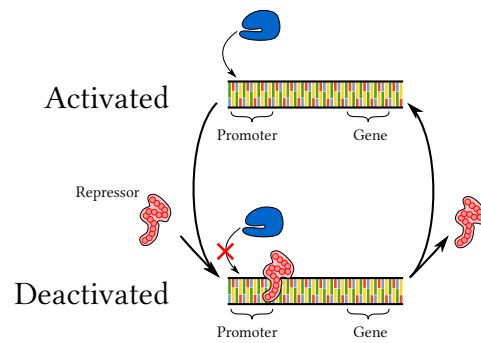
Figure 1.3: Gene activation and deactivation through a repressor.
