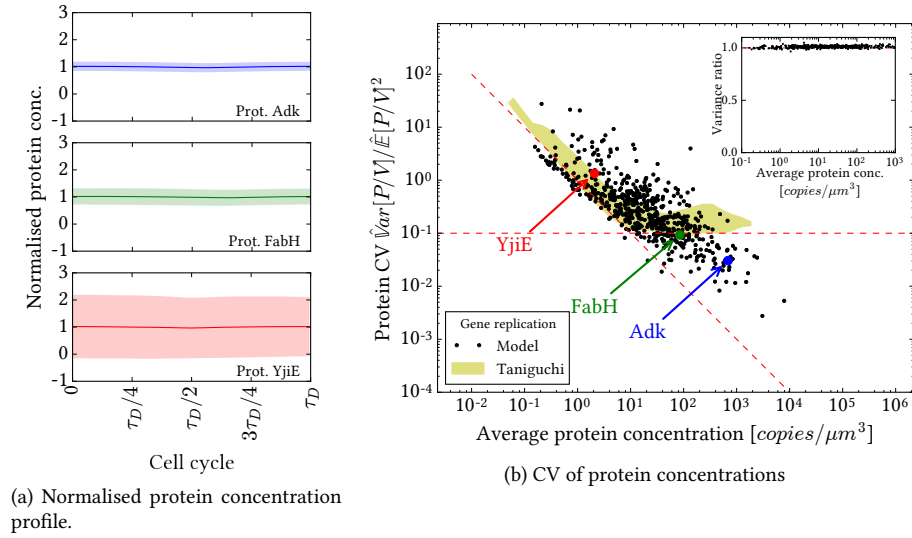
Figure 3.4: Result of simulations of the model with cell replication, compared with Taniguchi et al. (2010) experimentation. Figure 3.4a: normalised protein concentration profile over the cell cycle for three representative proteins. The thick line represents the mean concentration over the cell cycle, and the coloured area represents the standard deviation. The profile shows no significant differences with the previous models (see Figure 3.4a for the more details on Adk). Figure 3.4b: coefficient of variation (CV) of the protein concentration as a function of the average protein concentration. There are, once again, no significant differences as before (see Figure 3.4b ). In particular, there is no lower “extrinsic” noise plateau for highly expressed proteins, as it is the case for Taniguchi et al. (2010) (yellow area). Inset: ratio between the CV of protein concentration of the model with binomial sampling (Subsection 3.3.6) divided by the one of this section. Gene replication adds no particular noise compared with the model with only binomial sampling.
