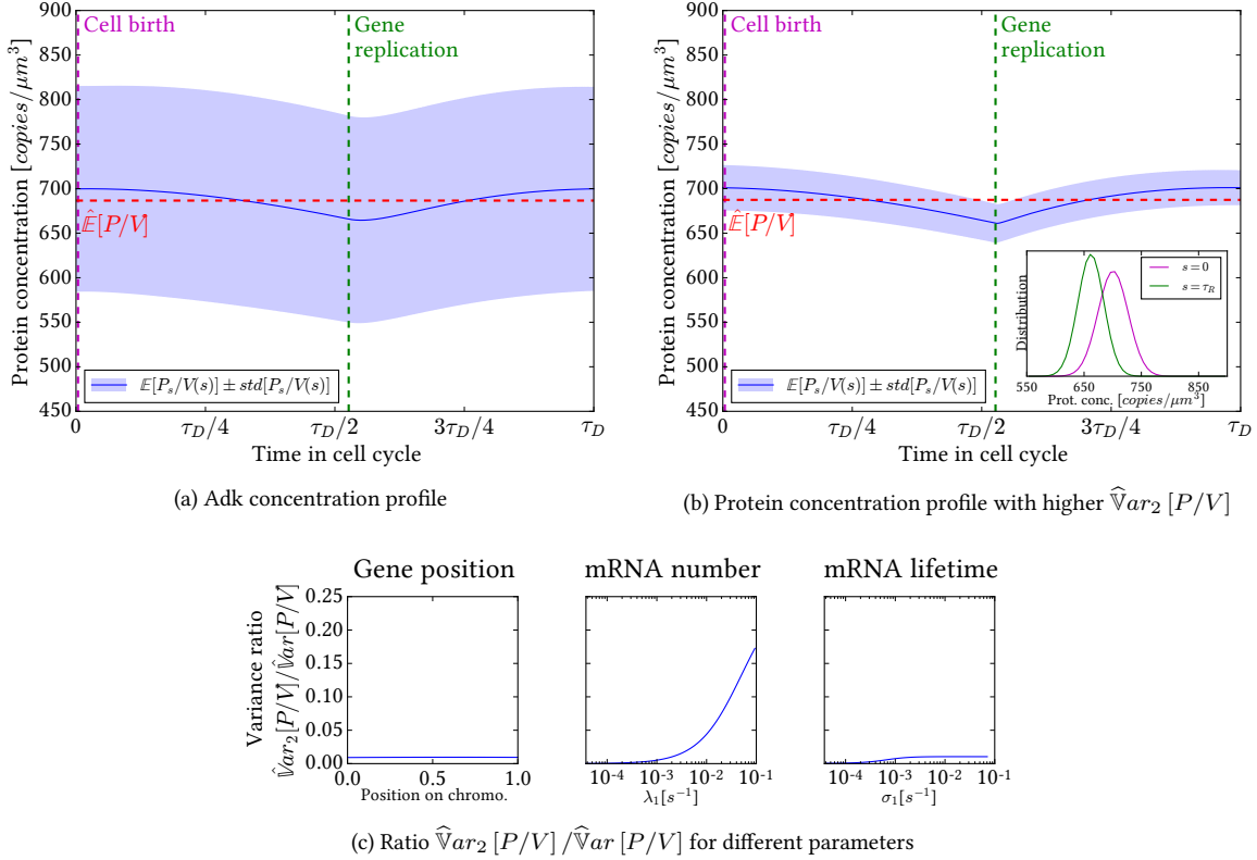
Figure 3.3: Protein profile. (a) : Protein profile concentration of Adk. The mean concentration \mathbb{E}[P_s/V(s)] is not constant across cell cycle and fluctuates across the global average \mathbb{E}[P/V] (in red). The large standard deviation of P_s/V(s) (coloured area) indicates a large term \widehat{\text{var}}_1[P_i/V] in the environmental state decomposition. (b) : profile of a modified version of AdK. In this version, there is a higher number of mRNAs (approximately ten times more) that last less time. The effect is a higher term \widehat{\text{var}}_2[P_i/V] in the environmental state decomposition (main figure), but it is not enough to clearly separate between the distributions at birth (at time s = 0 ) and at the replication of the gene (at time s = \tau_R ) (inset). (c) : Show the ratio \widehat{\text{var}}_2[P/V] / \widehat{\text{var}}[P/V] while varying successively the gene position, the mRNA number and the mRNA lifetime while keeping \mathbb{E}[P/V] constant.
