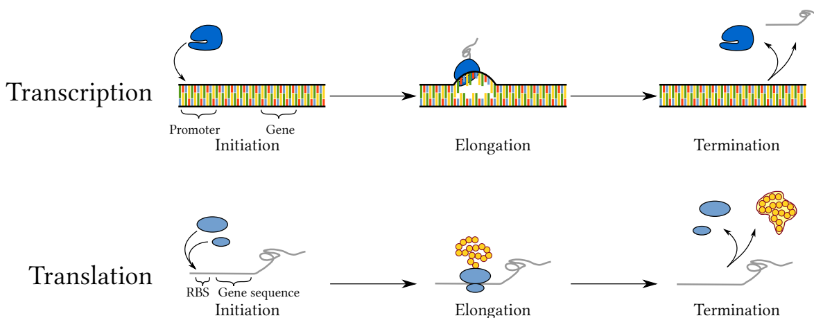
Figure 1.2: Schematic steps of transcription and translation
