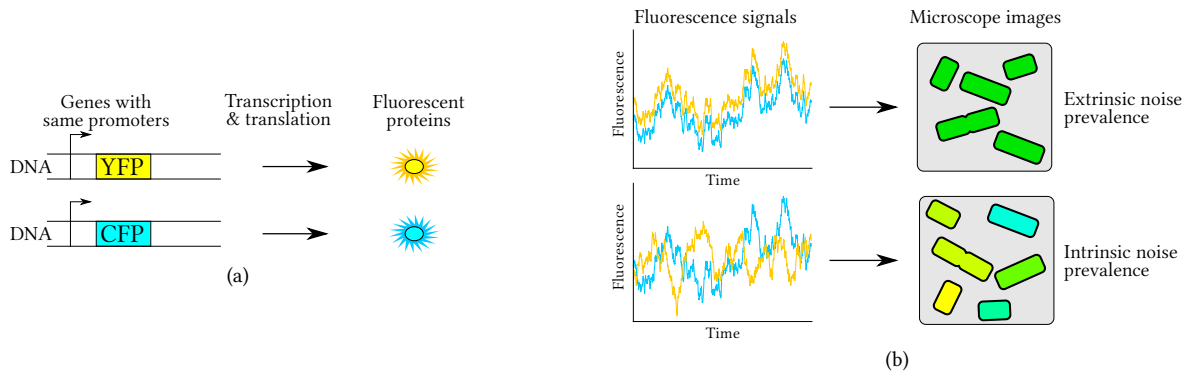
Figure 1.6: Dual reporter technique principle. (a): on the same chromosome, there are two genes with the same promoter, each coding for a fluorescent protein emitting a different wave length. (b): uncorrelated production give cells that express more of one of the fluorescent molecules. Above: a hypothetical situation showing fully correlated protein production; below: uncorrelated protein production (inspired by Elowitz et al. (2002) ).
