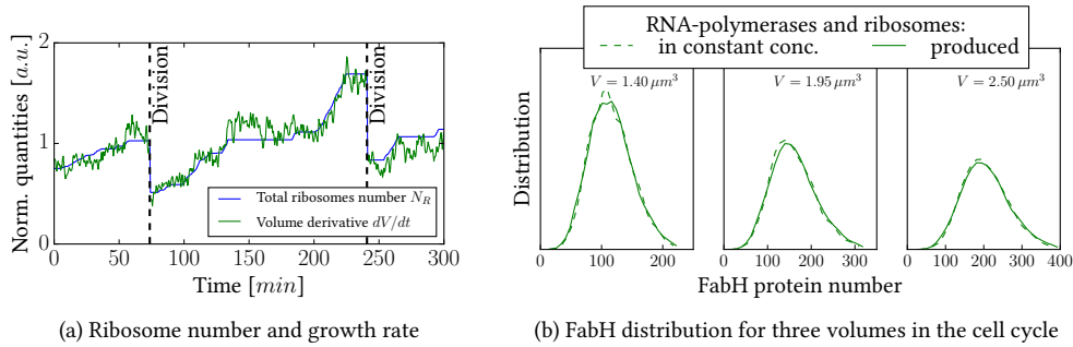
Figure 4.2: Model with production of RNA-polymerases and ribosomes. (a): correlation between the number of ribosomes and the growth rate in the modified version of the stochastic model. (b): distributions of the number of FabH protein for cells of volume 1.40 \mu\text{m}^3 , 1.95 \mu\text{m}^3 or 2.50 \mu\text{m}^3 . For each volume, the distribution in the model with production of RNA-polymerases and ribosomes is similar to the model with RNA-polymerase and ribosomes in constant concentration.
