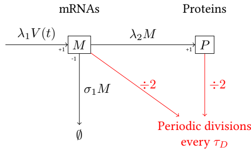
Figure 3.2: Model with cell cycle. (a) The model of this section considers genes independently from each other; the three mechanism of transcription, translation and division are represented. (b) For one particular type of protein, the number of mRNAs and proteins are respectively M and P (see main text for more details).
