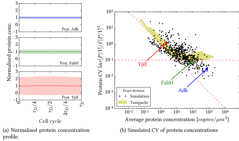
Figure 3.4: Result of simulations of the model with cell cycle, compared with Taniguchi et al. (2010) experiments. (a): Normalised protein concentration profile over the cell cycle for three representative proteins. The thick line represents the normalised mean concentration over the cell cycle \mathbb{E}[P_s/V(s)] , and the coloured areas represents the standard deviation. As predicted, the mean protein concentration remains constant over the cell cycle. Furthermore, we observe that the relative variance is higher for the less expressed proteins such as YjiE. (b): coefficient of variation (CV) of the protein concentration (defined as \hat{\text{var}}[P/V] / \hat{\mathbb{E}}[P/V]^2 ) as a function of the average protein concentration. It appears that the CV predicted by the simulation scales approximately inversely with the average protein production. Though, unlike Taniguchi et al. (2010) experiments, indicated by the yellow area (corresponding to the point cloud of Figure 3.1c), there is no lower plateau for highly expressed proteins.
