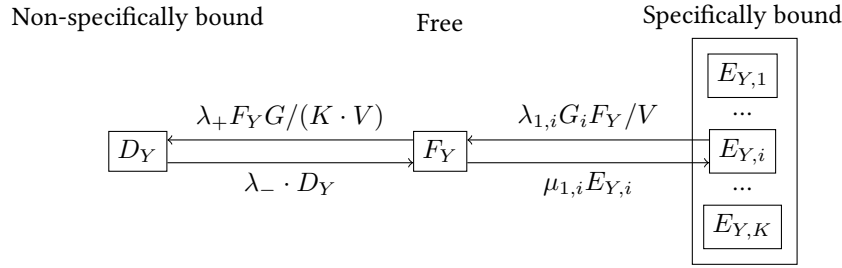
Figure 4.3: RNA-polymeses dynamics in the case of non-specific binding. An RNA-polymerses can be either among the specifically bound on the DNA (in E_{Y,i} for i \in \{1, \dots, K\} ) or free (among F_Y ) or non specifically bound on the DNA (among D_Y ).
