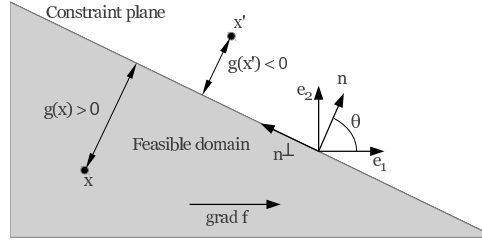
Figure 8.1: Linear function with a linear constraint, in the plane generated by \nabla f and \mathbf{n} , a normal vector to the constraint hyperplane with angle \theta \in (0, \pi/2) with \nabla f . The point \mathbf{x} is at distance g(\mathbf{x}) from the constraint.
