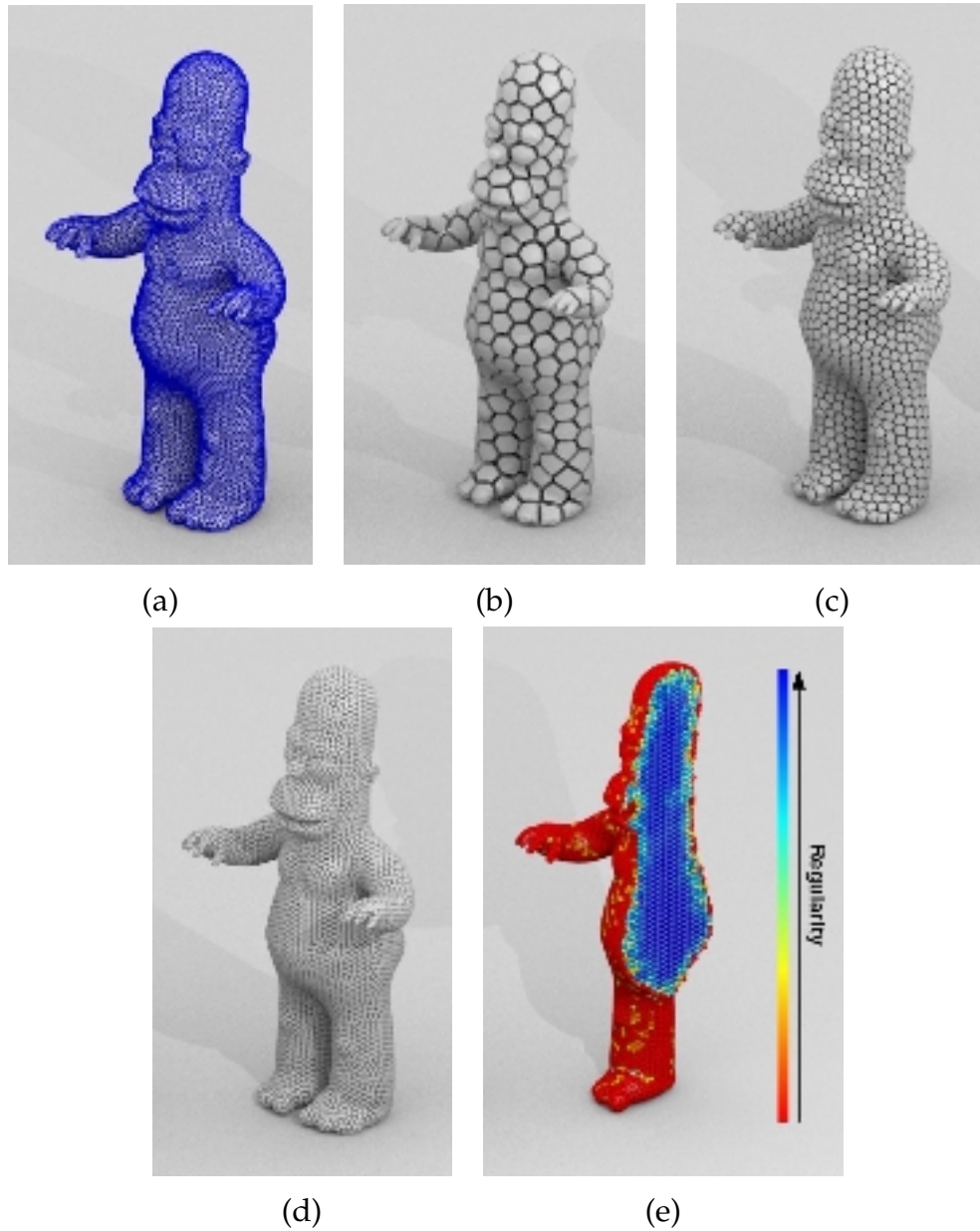
Figure 4.8 – Hierarchical CVT computation in 3D. (a) Input: a 3D shape bounded by a triangulated mesh. (b,c,d) Successive CVTs computed using our approach, with 546, 4375 and 35000 cells respectively. (e) A cut of Homer shows that most of the interior Voronoi cells present high regularity values.
