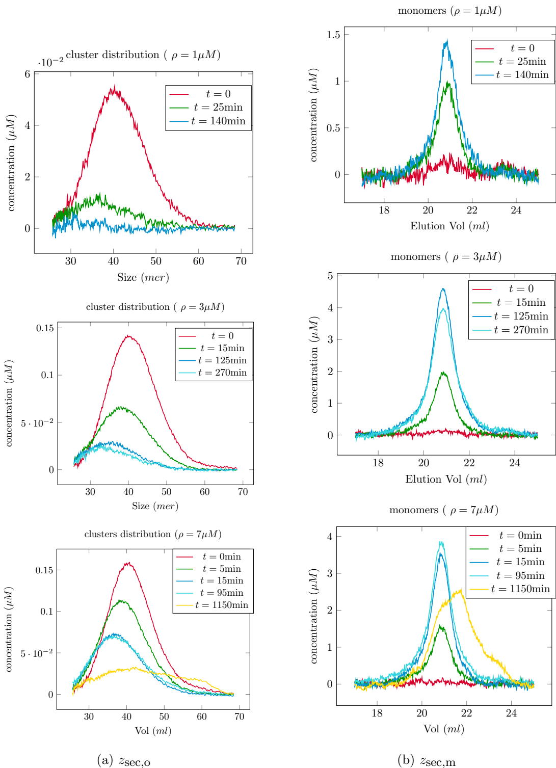
FIGURE 1.5 – Left : Oligomer distribution computed from SEC data. Right : monomer peak in SEC data. From the top to the bottom we consider the total concentrations \rho = 1, 3, 7 \mu M .
