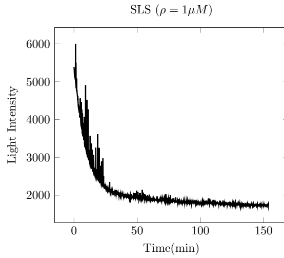
FIGURE 1.9 – SLS data at \rho = 1\mu M .
