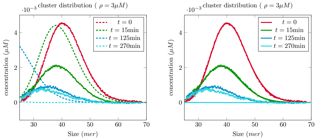
(a) Best fit of empirical size distribution data at \rho = 3\mu M with k_{\text{dis}_i} = 0 : parameters \mathcal{P}_1 = \{k_{\text{on}_i} = 0, k_{\text{dep}_i} = 0.16, k_{\text{dis}_i} = 0\} . (b) Best fit of empirical size distribution data at \rho = 3\mu M with k_{\text{dis}_i} \neq 0 : parameters \mathcal{P}_2 = \{k_{\text{on}_i} = 0, k_{\text{dep}_i} = 0.16, k_{\text{dis}_i} = 0.05\} .
