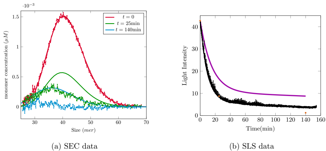
FIGURE 1.31 – Fit with the coefficients of Table T 1.3.8.1 relative to \rho = 1\mu M .
