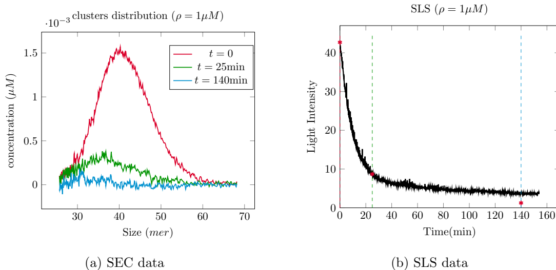
FIGURE 1.18 – Experimental data on ovPrP oligomer size distribution, total concentration \rho = 1\mu M .
