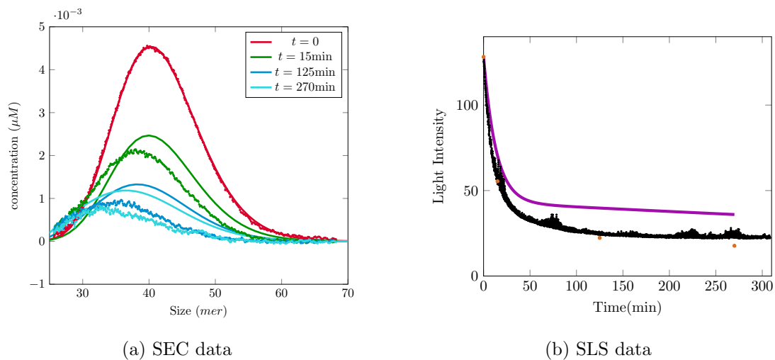
FIGURE 1.32 – Fit with the coefficients of Table T 1.3.8.1 relative to \rho = 3\mu M .
