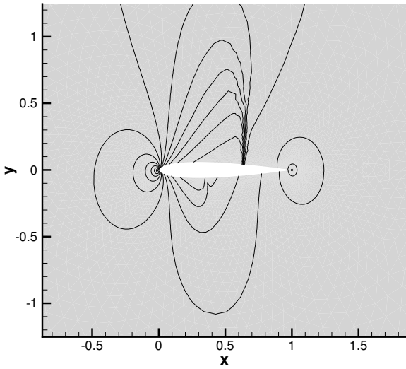
(a) Pressure ( \mathbb{P}^1 elements)
