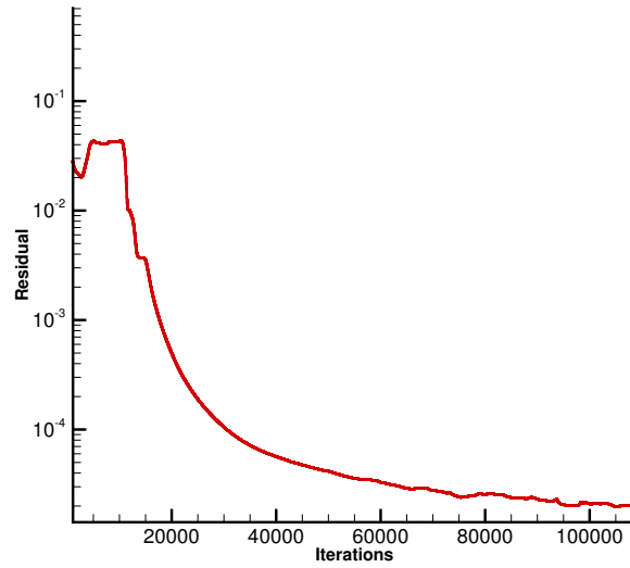
Figure 2.22: Convergence of residual for test case 2.4.4
