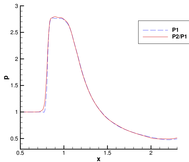
Figure 3.9: Comparison of pressure on line y = 1.44 with p-adaptation and P^1 elements.
