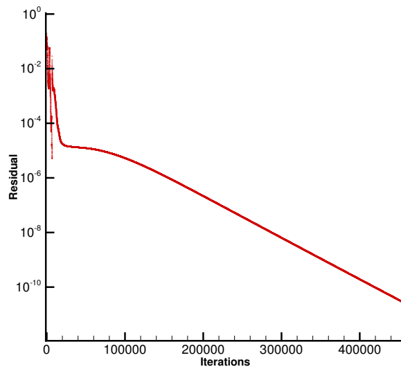
Figure 2.17: Convergence of residual for test case 2.4.3.
