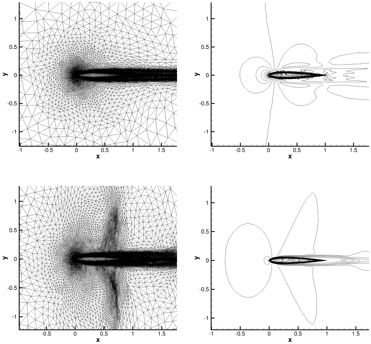
Figure 3.5: Final adapted meshes and solutions (Mach numbers) for test case 3.5.1 (subsonic and transonic regimes).
